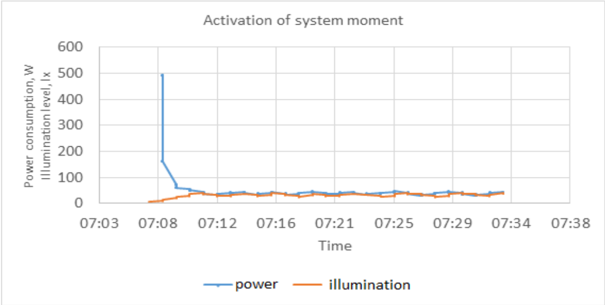
Fig. 17 Activation of the energy system prototype
