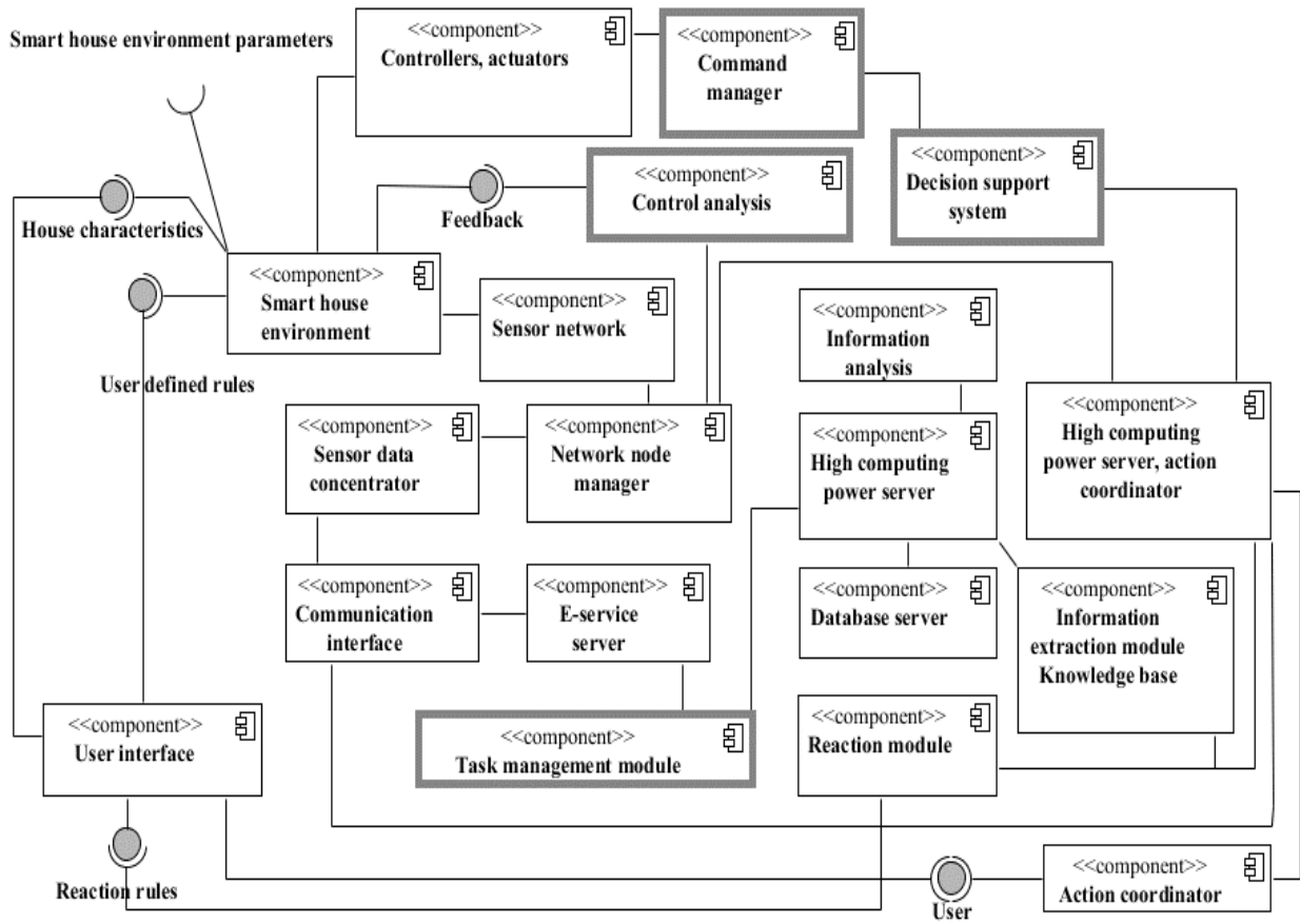
Fig. 9 Energy monitoring and decision support system
