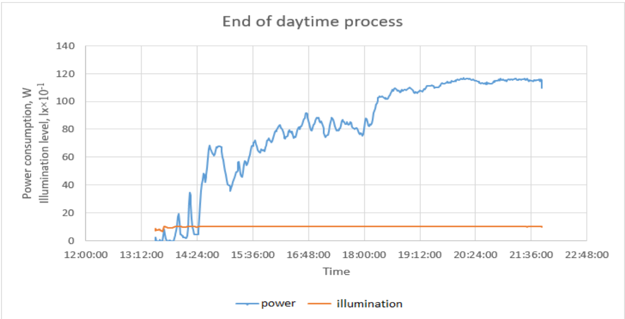
Fig. 18 Monitoring the process of the end of the daytime and autonomous management of illuminator
