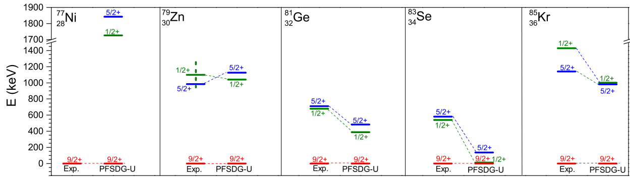
Fig. 5. Positive-parity levels in N = 49 isotopes due to neutron excitations across N = 50 , compared the calculated levels with the PFSDG-U interaction. The vertical dashed line in the 1/2^+ isomeric state of ^{79}\text{Zn} represents the error on the measured energy.
