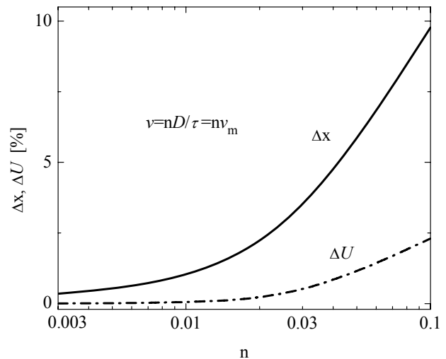
Fig. 3. The theoretic dependencies relative error of voltage determination and defective area center's coordinate determination. Scanning speed expressed as a part of maximal speed v_m = D/\tau ( \tau – time constant of measuring device).
