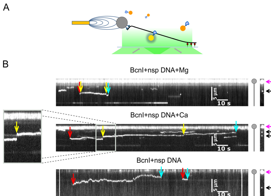
Figure 3. Observation of sliding and jumping of BcnI on DNA. (A) Experimental configuration. A 22.8 kb DNA molecule lacking BcnI recognition sites (black) was attached to a magnetic bead (grey sphere) and to the surface of a flow cell. The DNA was stretched sideways using a magnet placed next to the flow cell. An evanescent field (green) of a TIRF-microscope was illuminating quantum-dot labeled enzymes bound to the DNA (yellow). Most of the freely diffusing enzymes in solution (orange) were outside of the evanescent field. (B) Representative kymographs of the movement of quantum-dot labeled BcnI on the DNA in the presence of Mg^{2+} ions (top) (straight horizontal line in the lower part of the kymograph depicts protein stuck on the surface of the flow cell), in the presence of Ca^{2+} ions (middle), and without divalent metal ions (bottom). Protein association, jumps, and protein dissociation are marked with red, green and blue arrows, respectively. Positions of the magnetic bead and fluorescent BcnI proteins are marked on the right-hand side with magenta and black arrows, respectively.
