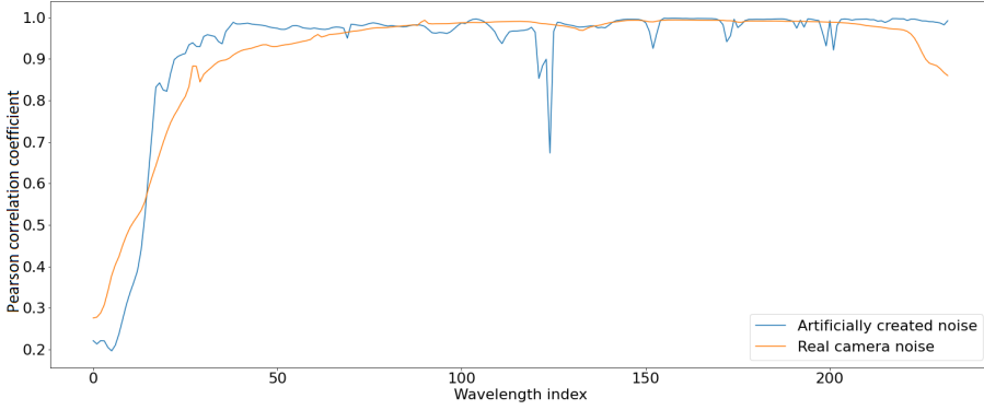
Figure 2.8 A comparison between the Pearson correlations of real and artificially created noise profiles.
