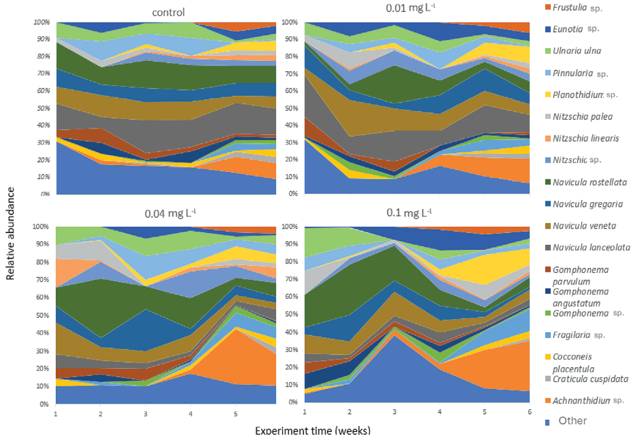
Fig. 5. Temporal variation in diatom abundance under different cadmium concentrations. Diatoms taxa comprising \geq 1\% of the total abundance per treatment are included.
