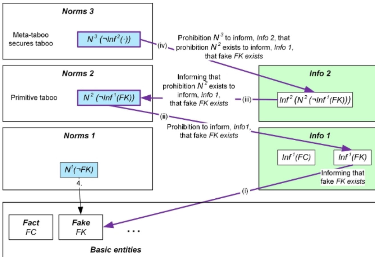
Figure 5: Meta-taboos Norms 3 and Info 2 added to Figure 4
