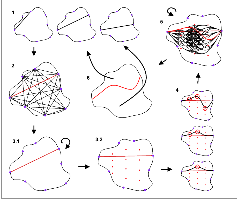
Figure 25. Visual workflow of the hespddiv algorithm process: (1) Construct multiple linear split-lines. (2) Assess each line’s effectiveness and select the optimal one (shown in red). (3) Based on the best linear split-line, generate nonlinear alternatives by: (3.1) rotating the polygon, and (3.2) creating a grid of spline control points. (4) Generate and assess multiple nonlinear split-lines. (5) Identify the final split-line. (6) Perform the split and iterate the process. Reproduced with permission from Daumantas and Spiridonov (2024b).
