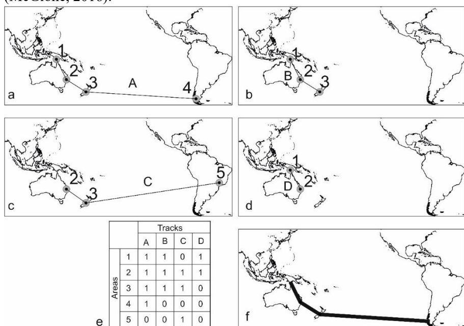
Figure 19. Tack compatibility analysis (Morrone & Crisci, 1995). From (a) to (d): tracks of different taxa. (e): An areas \times tracks matrix, indicating which areas each track passes through. (f): The generalised track derived from the numerical track compatibility analysis. Reproduced and modified with permission from (Morrone & Crisci, 1995). Coastlines data used in reproduction taken from Natural Earth (naturalearthdata.com).
