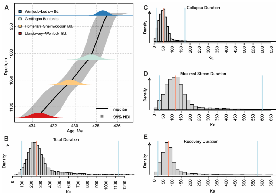
Figure 37. Bayesian age–depth model for the Gêluva-118 section (A), and estimated durations derived from it for (B) the entire Mulde/lundgreni event, and (C–E) its individual stages. The light-blue lines in panels B–E represent the 95% highest density interval (HDI), while the orange line indicates the median, i.e. the most probable duration. Reproduced from Rinkevičiūtė et al. (2025), licensed under CC BY 4.0 ( http://creativecommons.org/licenses/by/4.0/ ).
