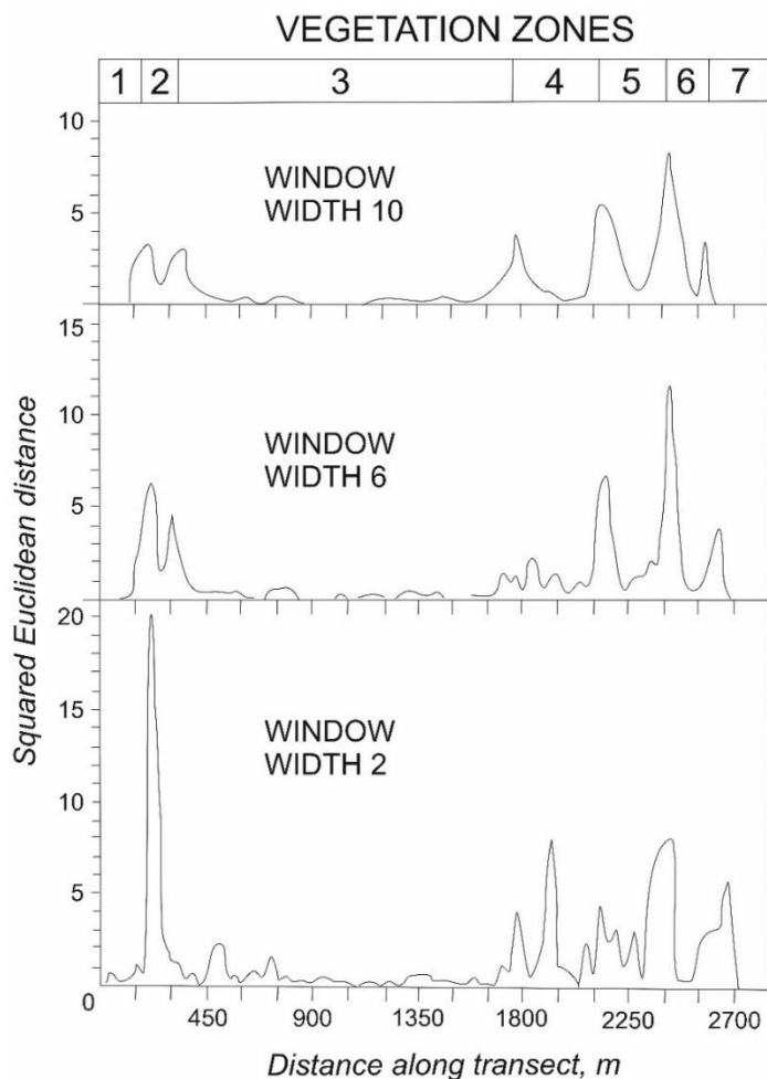
Figure 14. Example of SMW output, and how it depends on the scale of analysis (window width). The high peak obtained with a narrow window of width 2, represents an ecotone, whereas peaks visible using broader windows correspond to more fuzzy boundaries or ecoclines. Reproduced and modified with permission from Ludwig and Cornelius (1987).
