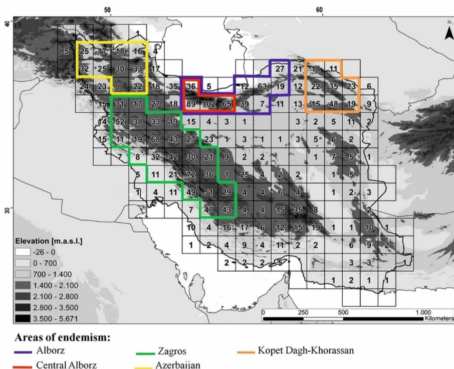
Figure 11. Endemic species richness of Asteraceae in Iran per grid cell, based solely on species occurring within the study area, with identified areas of
