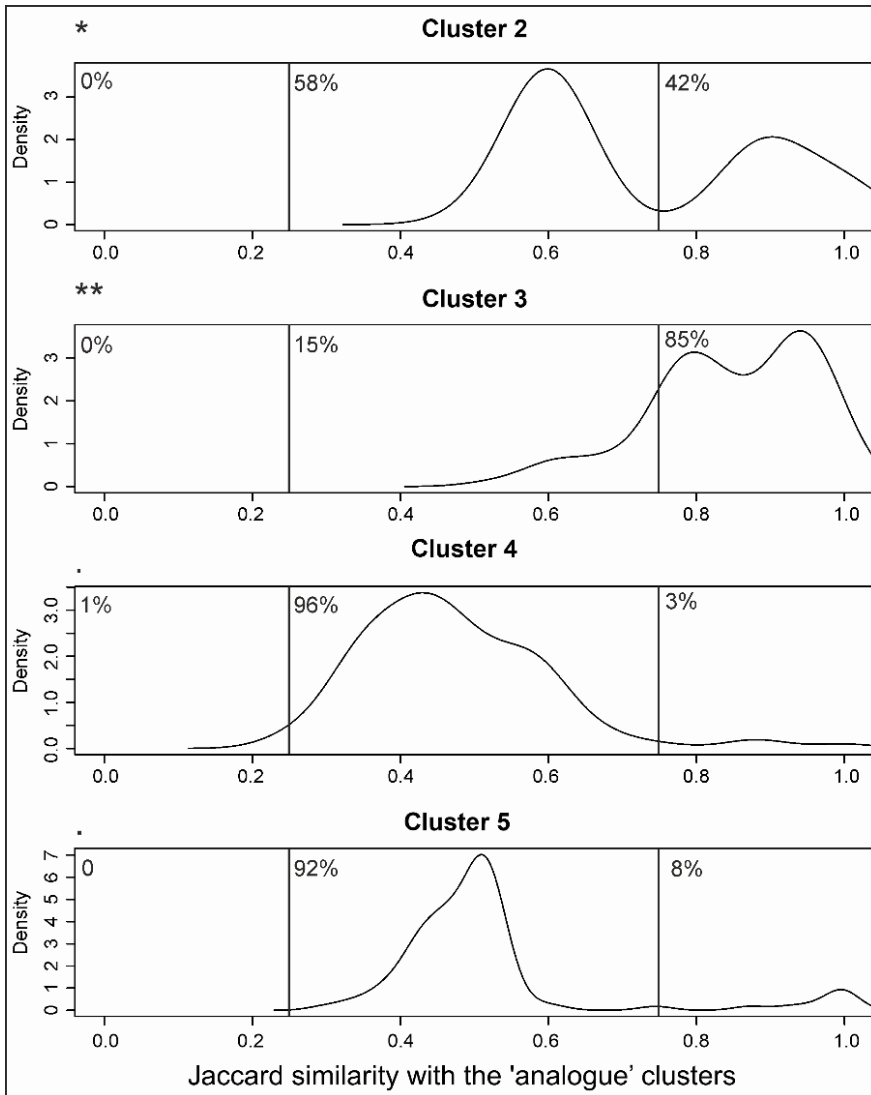
Figure 31. Stability of the 2nd to 5th HespDiv clusters illustrated by plotting empirical probability density functions (PDFs) of Jaccard similarity between the occurrences of established clusters and their most similar ‘analogue’ clusters identified in alternative subdivisions during the sensitivity analysis. Asterisks and dots indicate levels of HespDiv cluster stability: ** stable; * mostly stable; • somewhat stable (see Fig. 29 for definitions). Plots were generated using the plot_hsa_q() function. Stability results for clusters 6 to 29 are presented on the following two pages (figure continued). Reproduced with permission from Daumantas and Spiridonov (2024b).
