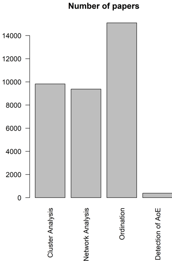
Figure 4. Number of Google Scholar search results (last checked on 8 April 2025) for the phrase “X” “biogeography”—where X is the method’s name—restricted to publications from 2020 onwards. The restriction was used to reflect contemporary trends. The acronym AoE stands for areas of endemism. The search phrase used for “Detection of AoE” was different, aggregating search results for three different methods: "biogeography" ("Endemism analysis") OR ("parsimony analysis of endemism") OR ("biotic element analysis").
