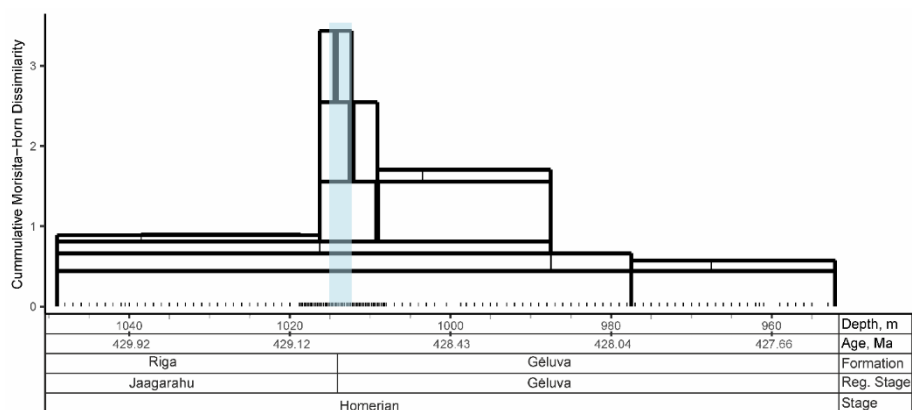
Figure 36. Hierarchical segmentation of ostracod assemblages from the Géluva-118 core. Each rectangle represents a stratigraphic segment defined by shifts in assemblage composition. The base rectangle encompasses the full section, with higher rectangles indicating further subdivisions. Vertical lines mark the split points of lowest Morisita–Horn similarity within each segment; their width and the rectangle height both reflect the degree of compositional dissimilarity ( 1 - \text{Morisita–Horn similarity} ). Taller and wider vertical lines indicate stronger contrasts. Cumulative dissimilarity values can be read on the vertical axis. Sampling positions are indicated by short ticks along the bottom. The light-blue zone marks the Maximal Stress stage. A ca. 80 cm offset between the Maximal Stress onset and the split of the tallest segment results from the requirement that segments include a minimum of 10 samples—an artefact that only affects narrow, sparsely sampled intervals and does not influence the broader delineation of the Mulde/lundgreni Event. Reproduced from Rinkevičiūtė et al. (2025), licensed under CC BY 4.0 ( http://creativecommons.org/licenses/by/4.0/ ).
