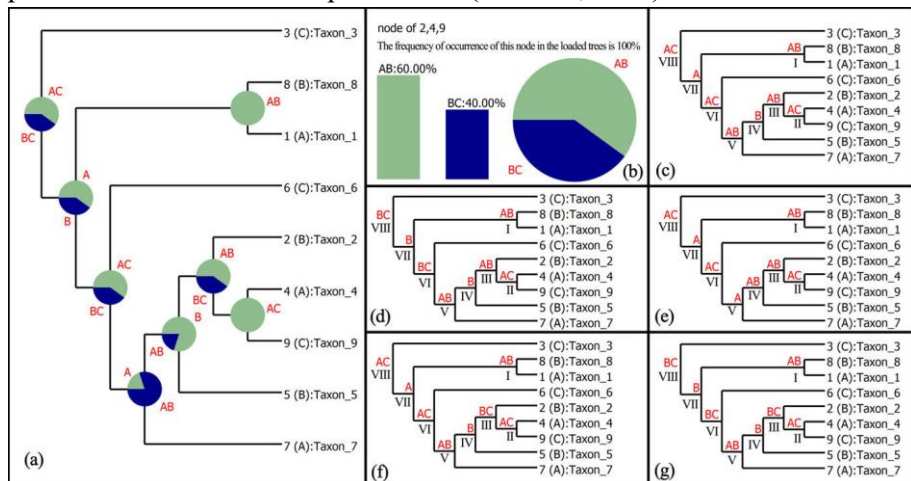
Figure 22. Graphical S-DIVA output as presented in Yu et al. (2010), reproduced with a permission. (a) Ancestral distributions for a simulated 9-species phylogeny across 3 areas (A, B, C), with pie charts showing probabilities of alternative ancestral ranges at nodes. (b) The node ((4,9),2) has two possible ancestral ranges (AB: 60%, BC: 40%), displayed as pie and bar charts in S-DIVA; since the node appears in all trees, its probability is 100%. (c–g) Five optimal reconstructions contributing to the probability estimates in (a) and (b).
