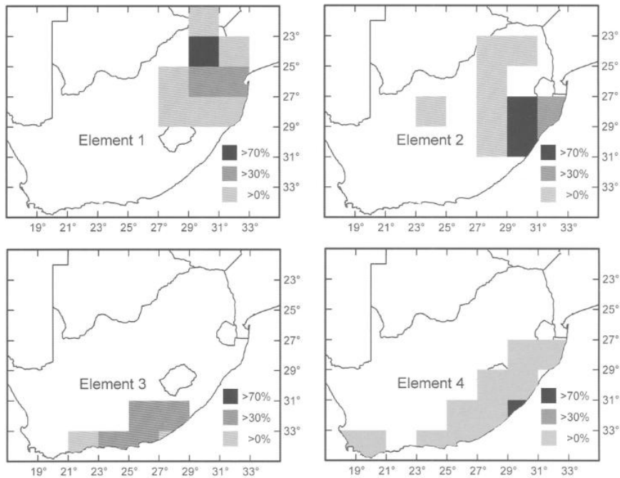
Figure 12. Distribution maps of four biotic elements based on the mapped ranges of South African Scobius species on a 2° grid (with some Namibian grid squares omitted). Shading indicates areas where more than 70%, more than 30%, and more than 0% of an element's species are present. Reproduced with permission from Hausdorf and Hennig (2003).
