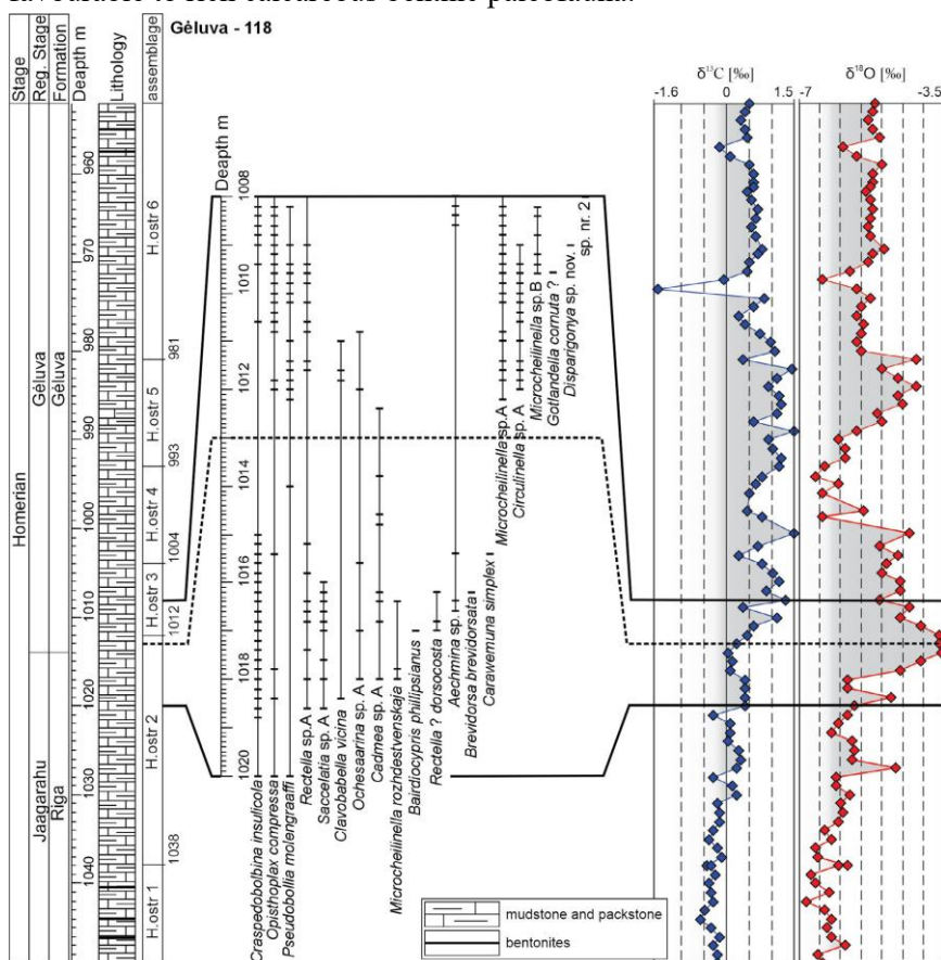
Figure. 34. The stratigraphic distribution of lithology, ostracod occurrences, and statistically significant (99% level) ostracod assemblage compositions is shown alongside carbonate \delta^{13}\text{C} and \delta^{18}\text{O} trends. Reproduced from Rinkevičiūtė et al. (2025), licensed under CC BY 4.0 ( http://creativecommons.org/licenses/by/4.0/ ).
