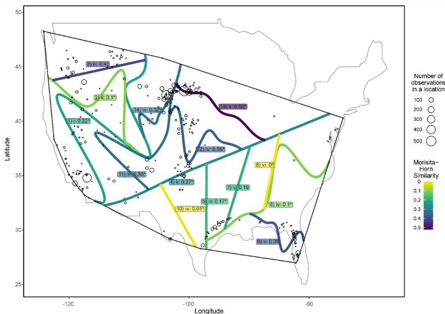
Figure 27. The map generated by applying the plot_hespddiv() function to the results. It illustrates the hierarchical subdivisions derived from the US Miocene mammalian assemblage data. Each split-line is labelled with its identification number (indicating the sequence in which it was derived), its hierarchical rank (denoted in Roman numerals), and the Morisita–Horn similarity value, which is also represented by colour. Statistically significant split-lines are marked with an asterisk. The size of each circle on the map corresponds to the number of taxa recorded at that fossil locality. Reproduced with permission from Daumantas and Spiridonov (2024b).
