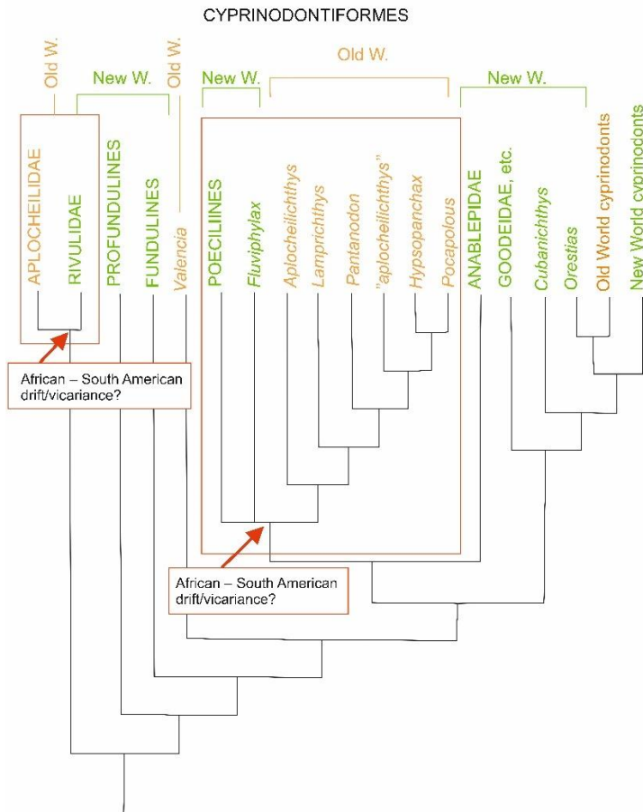
Figure 20. This area cladogram, based on phylogenetic hypotheses by Parenti (1981), illustrates the biogeographic history of Cyprinodontiformes. Red rectangles denote groups whose biogeographic history is best explained by African–South American drift-induced vicariance. In contrast, explaining the biogeographic history of other groups requires the consideration of over-oceanic marine dispersal. For example, while the African–South American separation accounts for the distribution of Poeciliidae in South America and Aplocheiloidei in Africa, the occurrence of younger aplocheilid groups outside Africa (e.g. Pantanodon ) suggests that marine dispersal events have also played a role after the fragmentation of Gondwana (Lundberg, 1993). Figure reproduced and modified with permission from Lundberg (1993).
