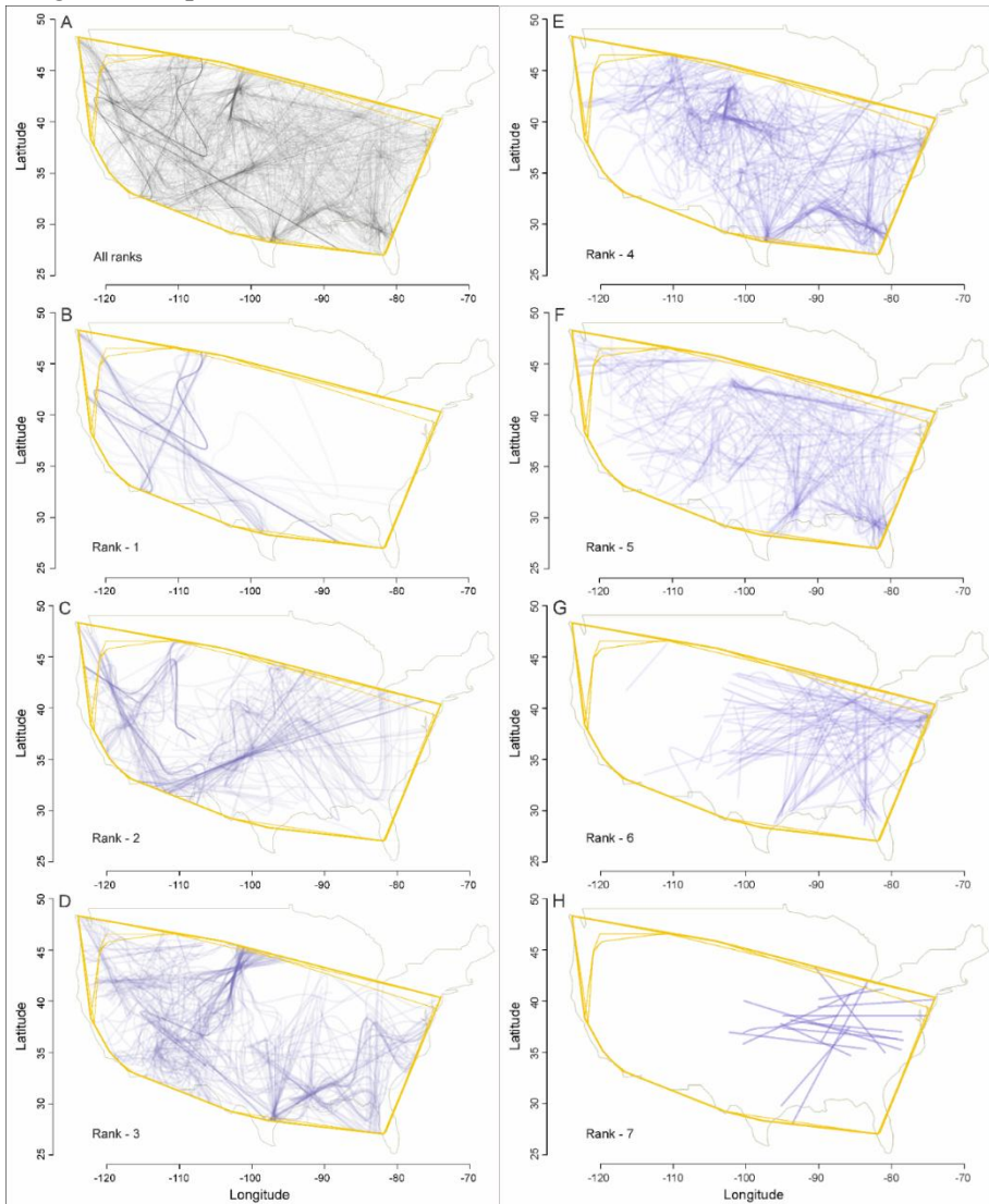
Figure 30. Stability of HespDiv polygons illustrated by plotting split-lines from all alternative subdivisions produced in the hespdiv sensitivity analysis. The plots were generated using the plot_hsa() function. Panel A shows all ranks combined, while panels B to H display split-lines ranked from 1 to 7, respectively. Reproduced with permission from Daumantas and Spiridonov (2024b).
