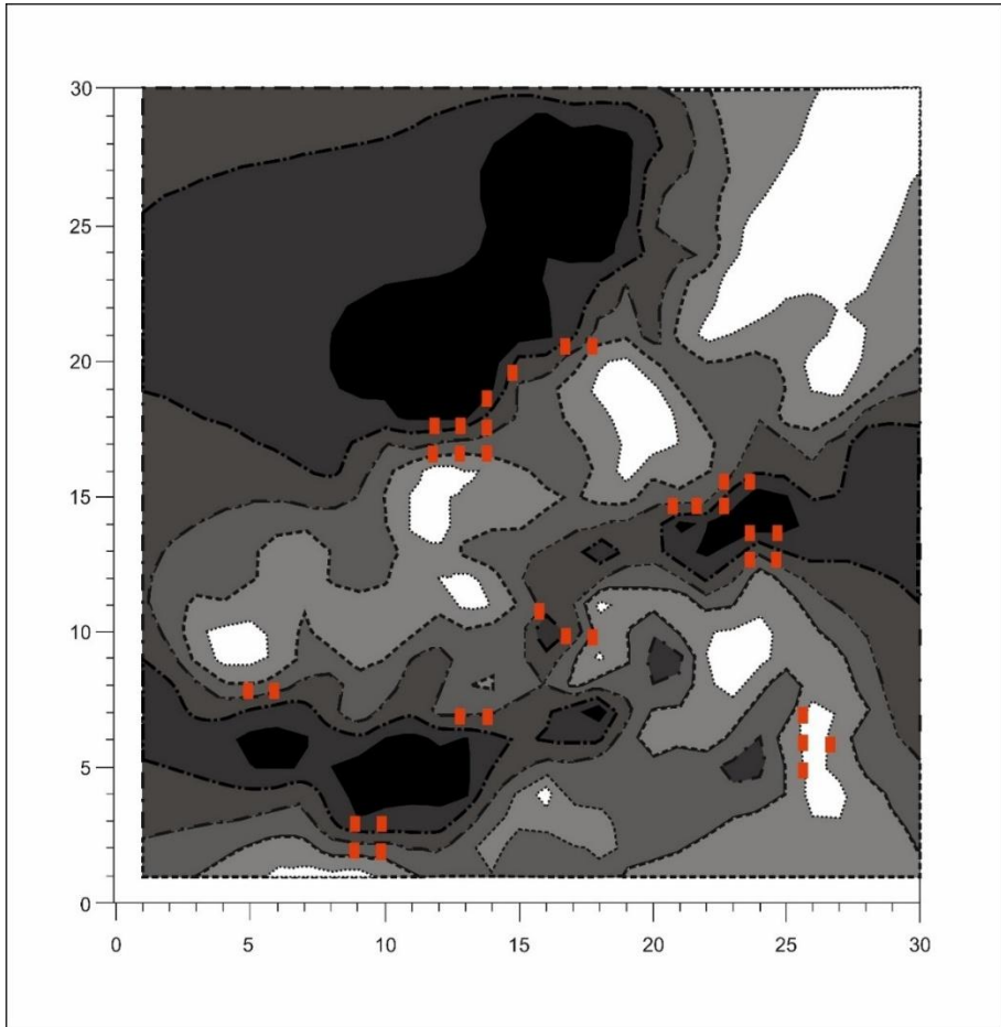
Figure 16. Map of the Swiss Jura region showing wombling boundaries (red rectangles) detected in cobalt concentrations. Map covers 30x30 grid over 14.5 km 2 geographic region. The boundaries were tested for significance using a Monte Carlo approach, employing the mean boundary length as a test statistic. Boundaries are superimposed on a kriging interpolation map. Reproduced and modified with permission from Gleyze et al. (2001).
