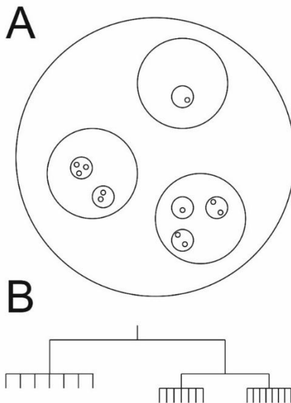
Figure 2. A – compositional hierarchy, B – Control hierarchy. Recreated modified after Salthe (1985).
