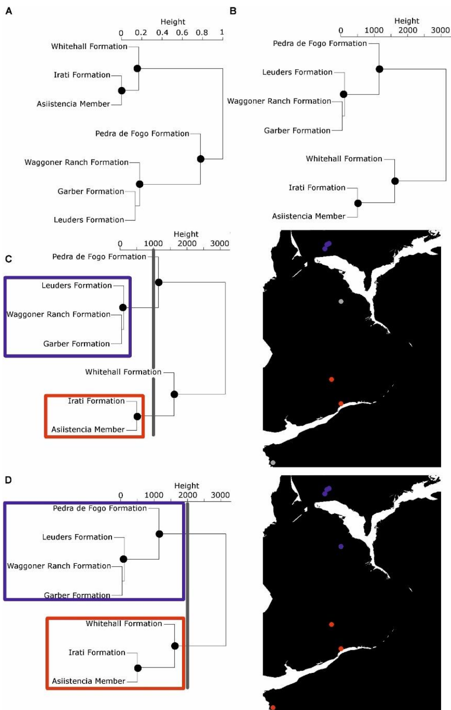
Figure 5. The example of various hierarchical cluster approaches using early Kungurian tetrapod data. (A) classical UPGMA dendrogram based on taxonomic dissimilarities between formations. (B) Dendrogram of the same
