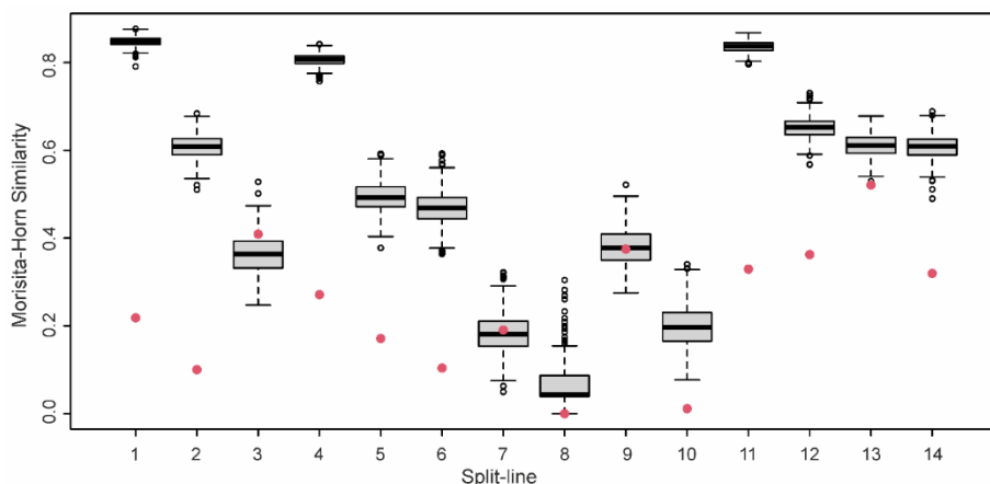
Figure 28. Statistical significance of split-lines assessed using the nulltest() function. Red dots represent the original empirical performance of each split-line, while the boxplots illustrate the distribution of performance values generated from 500 randomised reshufflings of the occurrences. Reproduced with permission from Daumantas and Spiridonov (2024b).
