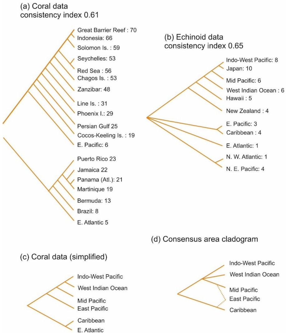
Figure 10. Cladograms of sample localities based on PAE analysis for extant reef coral and clypeasteroid echinoid genera. (a) Detailed coral data area cladogram, (b) Detailed echinoid area cladogram, (c-d) simplified consensus cladograms. Numbers following locality names in a-b indicate the count of genera shared with at least one other locality. Reproduced and modified with permission from B. R. Rosen (1988).
