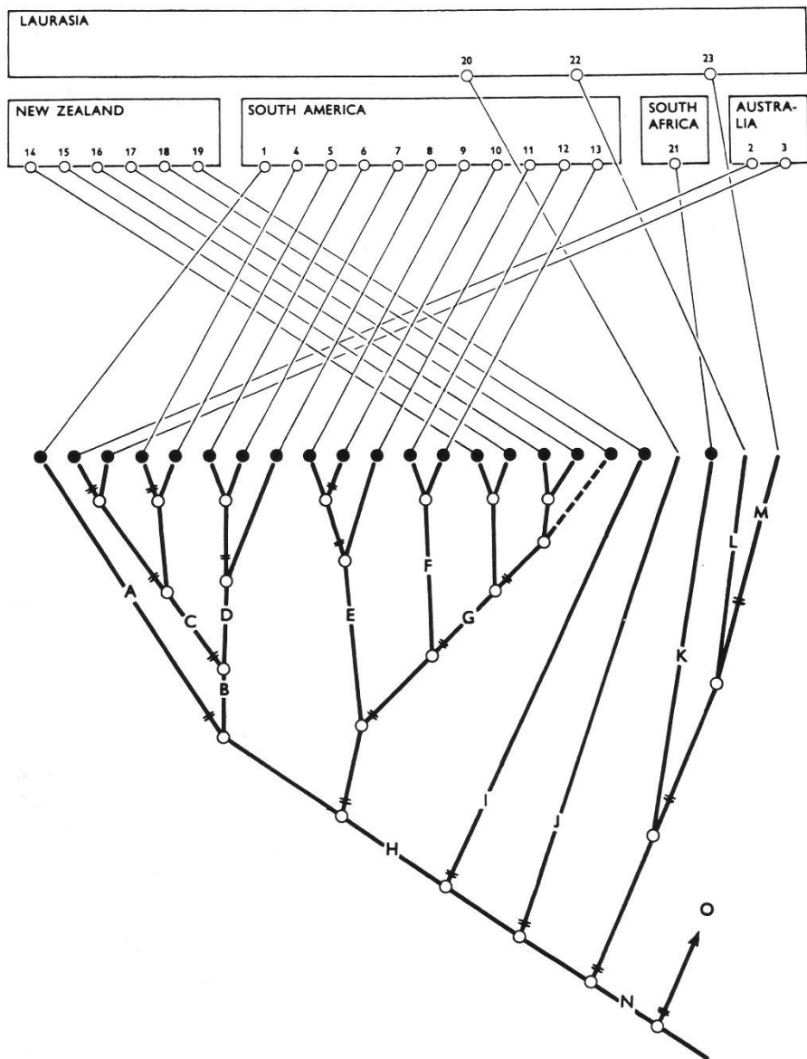
Figure 18. Phylogenetic tree of the Diamesinae and their geographic distribution (Brundin, 1966). Applying a phylogenetic biogeography approach to this pattern led to the interpretation that South America and New Zealand each had separate connections with Antarctica, while South Africa was the first landmass to lose all connections. Additionally, Australia was identified as the centre of evolution (Morrone, 2023). Reproduced from Morrone (2023), licensed under CC BY 4.0 ( http://creativecommons.org/licenses/by/4.0/ ).
