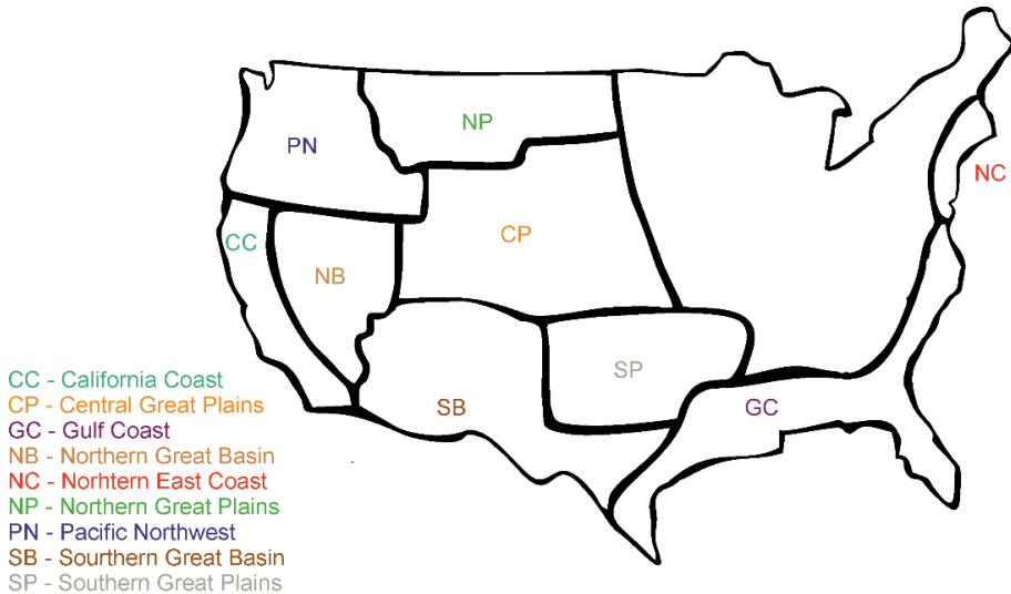
Figure 33. Bioregionalisation scheme of North American Tertiary mammals as proposed by Janis (1998), originally derived from Tedford et al. (1987). For easier comparison with Fig. 27, the map has been cropped to match the extent of the contiguous United States. Reproduced with permission from Daumantas and Spiridonov (2024b).
