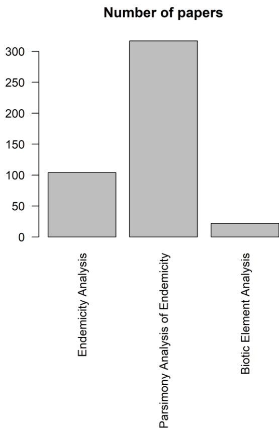
Figure 9. Number of Google Scholar search results (last checked on 8 April 2025) for the phrase ““X” “biogeography””—where X is the method’s name—restricted to publications from 2020 onwards. The sum of all papers here is higher than in aggregated result in Fig. 4 since some studies were comparative, applying more than one method to detect areas of endemism.
