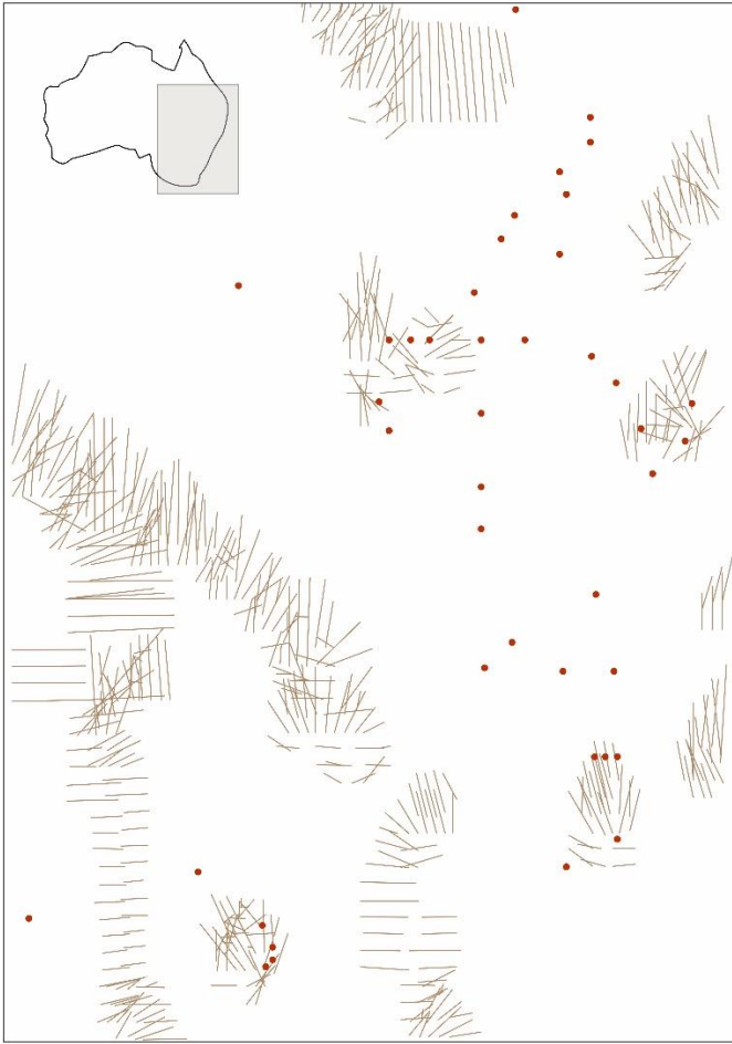
Figure 15. Boundaries produced by lattice wombling, based on the average orientation and magnitude of maximum rates of change in the frequencies of nine alleles in Australian Drosophila buzzatii . Boundaries are oriented perpendicular to the displayed rods, with rod length indicating boundary strength. Here, rods representing boundaries in the highest decile and ‘bridge’ boundaries in the second-highest decile of average turnover rates are shown. Dots represent locations of the studied Drosophila populations. The SYMAP interpolation algorithm was employed to create the regular grids required for lattice wombling. Note that identified boundaries are concentrated around the peripheries of the central distribution of locations, and several areas exhibit increased spatial heterogeneity in allelic frequencies. Furthermore, two larger bioregions could be inferred from these boundaries: one wedge-shaped region in the southwest and another located to its northeast. Rectangle at the top represent the study area location within Australia. Reproduced and modified with permission from Barbujani, et al. (1989).
