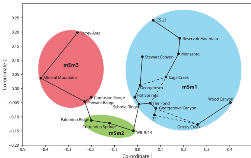
Figure 7. Example of ordination method (non-metric multidimensional scaling, NMDS) applied for bioregionalisation purposes on ammonoid faunas from Early Triassic, Western USA Basin. Most frequently recovered NMDS configuration (appearing in 378 out of 500 iterations, or 75%) shown with a
