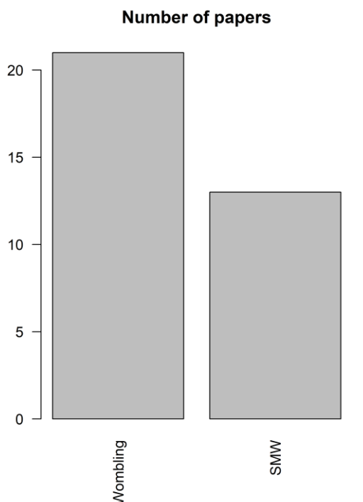
Figure 13. Number of Google Scholar search results (last checked on 8 April 2025) for the phrase “X” “biogeography”—where X is the method’s name—restricted to publications from 2020 onwards. Since split moving-window (SMW) is sometimes referred to as moving split-window (MWS), the searching phrase used was: "biogeography" ("Split Moving Window" OR "Moving Split Window").
