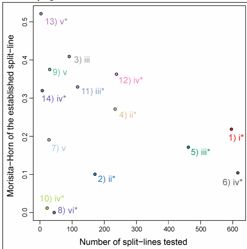
Figure 32. Relationship between the number of linear split-lines tested and the rank, comparison score, and statistical significance of the selected split-line. As in Fig. 27, each split-line is labelled with its identification number, rank (in Roman numerals), and an asterisk indicating statistical significance; colours correspond to those used in Fig. 29. Reproduced with permission from Daumantas and Spiridonov (2024b).
