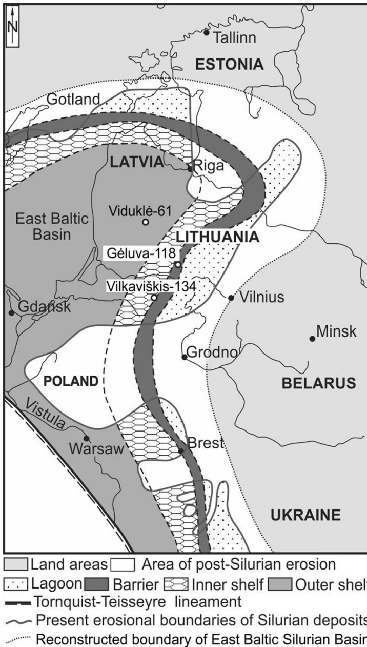
Figure 35. Location of the Gėluva-118 core and palaeogeographic reconstruction of the surrounding areas. The location of the Viduklė-61 core, which was important in establishing Gėluva-118 core geochronology via graphical correlation, is also shown. Map reproduced from Rinkevičiūtė et al. (2022).
