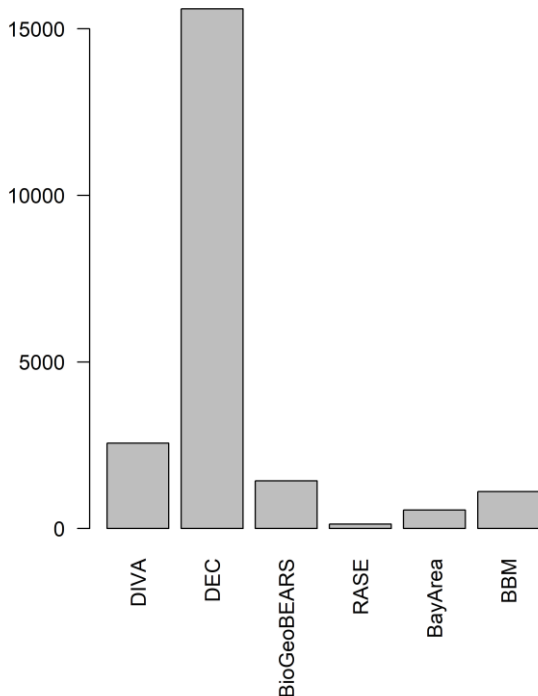
Figure 21. Number of Google Scholar search results (last checked on 12 March 2025) for the phrase “X” “biogeography”—where X is the method’s name—restricted to publications from 2020 onwards. The restriction was used to reflect contemporary trends. Full names of the methods are Dispersal-Vicariance Analysis (DIVA), Dispersal-Extinction-Cladogenesis modelling (DEC), BioGeography with Bayesian (and likelihood) Evolutionary Analysis in R scripts (GeoBioBEARS), Range Ancestral State Estimation (RASE), Bayesian inference of historical biogeography for discrete areas (BayArea), Bayesian Binary Monte Carlo Markov Chain Analysis (BBM).
