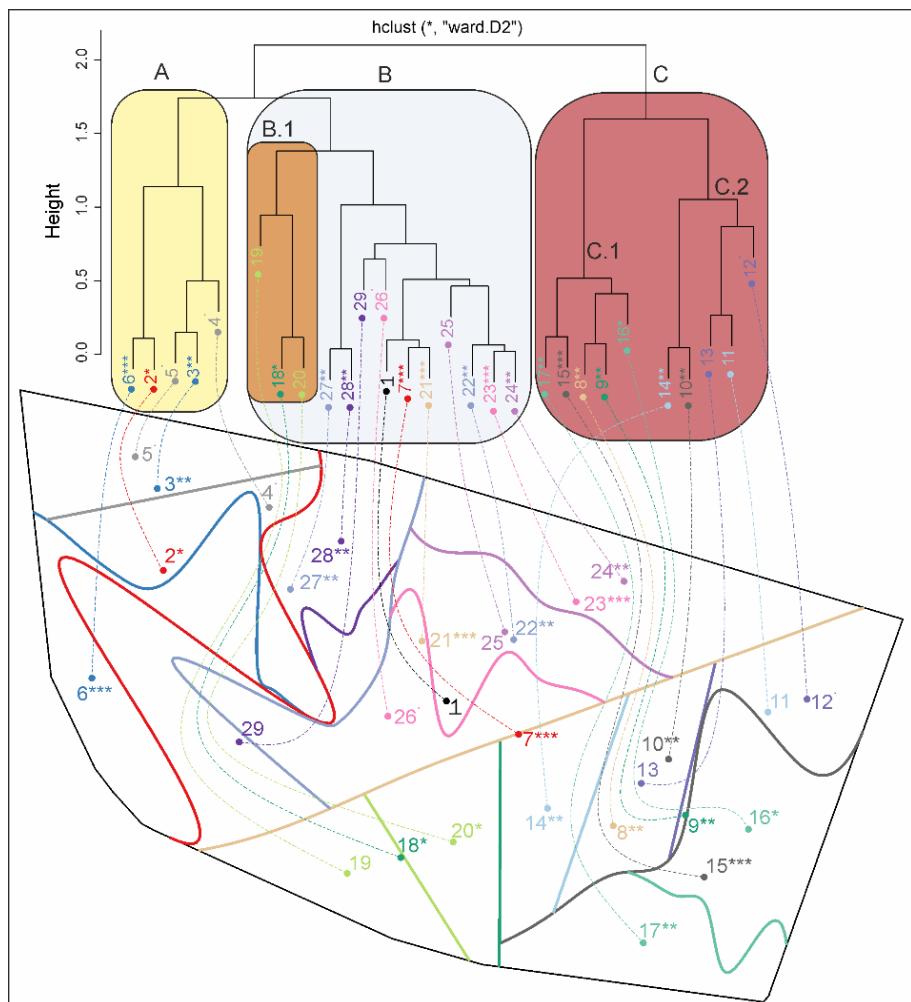
Figure. 29. Relationships among HespDiv polygons illustrated through a cluster dendrogram. The lower section of the figure shows the HespDiv polygons, visualised using the poly_scheme() function, while the upper dendrogram was generated by applying hierarchical cluster analysis to a distance matrix derived from the output of the cross_comp() function. Each polygon is represented by its centroid, label, and the colour of the split-line that generated it. Cluster stability, as determined through sensitivity analysis, is categorised into five levels and indicated using asterisks or a dot: *** very stable—more than 95% of alternative subdivisions produced a closely matching 'analogue' cluster (with Jaccard similarity \geq 0.75 ); ** stable—at
