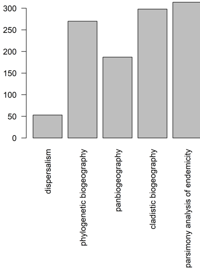
Figure 17. Number of Google Scholar search results (last checked on 12 March 2025) for the phrase “X” “biogeography”—where X is the method’s name—restricted to publications from 2020 onwards. The restriction was used to reflect contemporary trends.
