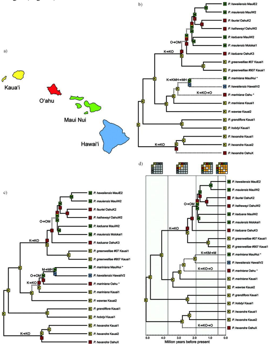
Figure 23. Example output from a DEC analysis in an empirical case study investigating the historical biogeography of Psychotria in the Hawaiian Islands. (A) Map showing the islands included in the study. (B–D) Ancestral range reconstructions: (B) using an unconstrained DEC model; (C) using a constrained DEC model, allowing only eastward dispersal and restricting area definitions to combinations of up to two adjacent islands, this model yielded the highest likelihood; and (D) using a temporally stratified DEC model,
