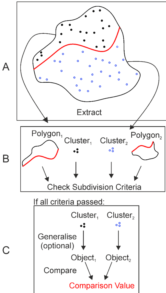
Figure 26. Visual representation of the three-step process for evaluating split-line performance: A – A split-line (red) divides the occurrence dataset and its polygon into two separate parts. B – The resulting subsets are checked to ensure they meet the required subdivision criteria. C – The subsets are then compared using a specific subdivision method by applying a combination of generalization and comparison functions to filtered datasets. Reproduced with permission from Daumantas and Spiridonov (2024b).
