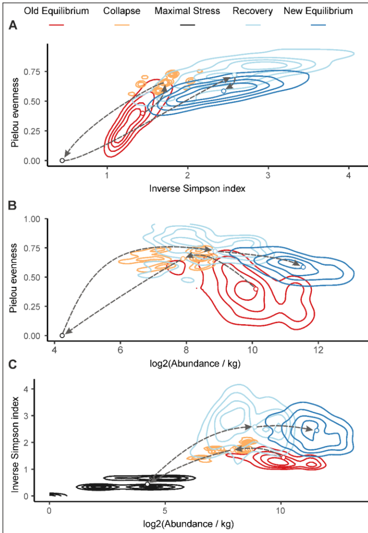
Figure 38. Contour plots showing bootstrapped sample means of diversity indices for ostracod populations at successive stages of the Mulde/ lundgreni event. Points mark the centroids of the distributions, connected by arrows indicating chronological progression. Each stage is represented by four contour lines, dividing the range of empirical probability density distribution into five equal intervals. Reproduced from Rinkevičiūtė et al. (2025), licensed under CC BY 4.0 ( http://creativecommons.org/licenses/by/4.0/ ).
