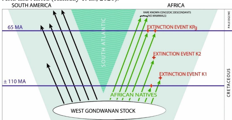
Figure 3. Diagram illustrating the macroevolutionary histories of South American and African faunas after their separation. Reproduced with permission from Rage and Gheerbrant (2020).
