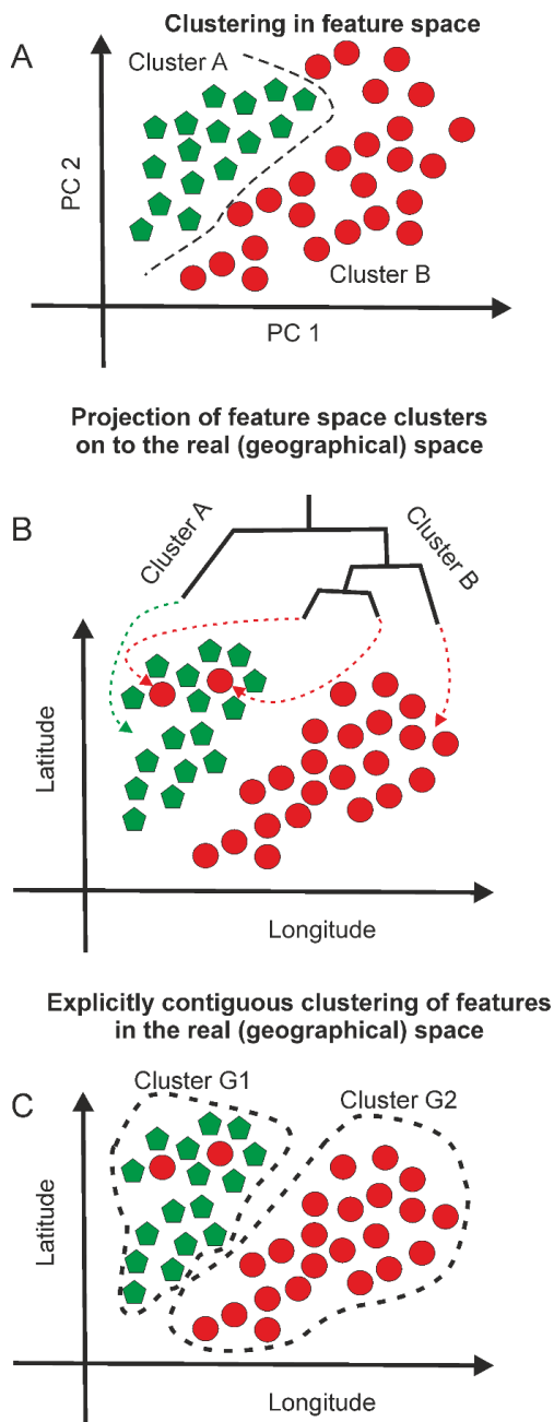
Figure 6. A) Cluster analysis conducted in feature space, such as the space of taxonomic compositions of palaeocommunities, groups or divides samples based solely on their similarities or differences, without accounting for their geographical positions. B) When these clusters are subsequently mapped onto geographical space, the resulting spatial representations are often non-contiguous, thereby violating the principles of spatially nested hierarchies. C)
