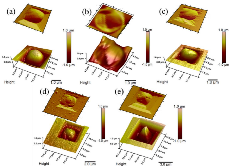
Figure 4. AFM images show: (a) an unmodified yeast cell; (b) an inactivated yeast cell; (c) a yeast cell modified with pPy at a concentration of 0.05 mM; (d) a yeast cell treated with pPy at a concentration of 0.1 mM; and (e) a yeast cell modified with pPy at a concentration of 0.3 mM. Originally from A. Zinovičius 2022 y. publication. 170
