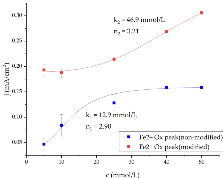
Figure 19. Current density dependencies on glucose concentration extracted from [\text{Fe}(\text{CN})_6]^{4-} peaks in CV. 200 mM pyrrole-modified and non-modified yeast used in the experiments, fitted using Hill's equation (Equation 2).
