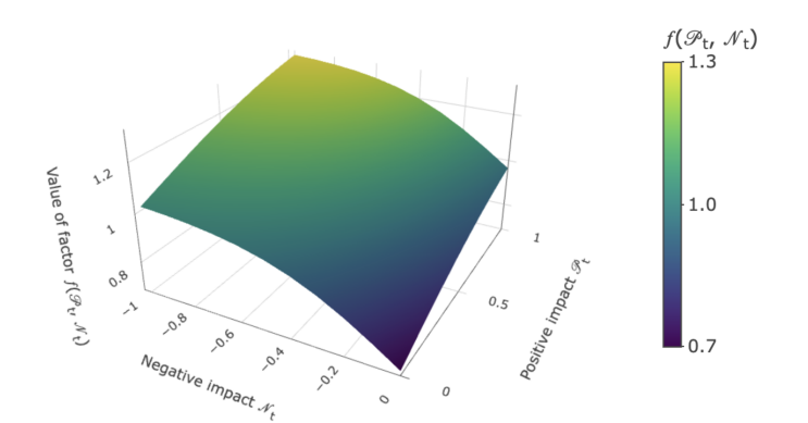
Figure 1. Surface plot of the news function f(\mathcal{P}_t, \mathcal{N}_t) of positive ( \mathcal{P}_t ) and negative ( \mathcal{N}_t ) news indices, showing the nonlinear response to news shocks for parameter values a = 0.7 , b = 0.7 , \kappa = 2 , and \gamma = 4 .
