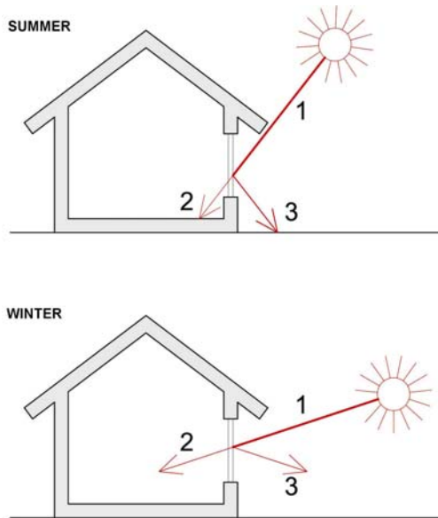
Fig. 2. Solar energy gains through south glazing depend on solar height above the horizon. 1 – solar energy reaching the glazing, 2 – solar energy penetrating the building, 3 – reflected solar energy
