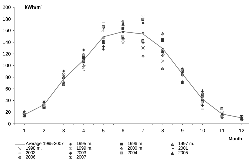
Fig.1. Average global solar radiation on the horizontal plate in Vilnius, monitoring data for 1995-2007 period
