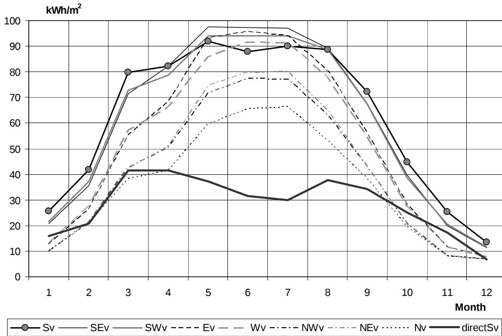
Fig 3. Total solar radiation and direct solar radiation to different orientations of vertical plane. Sv, SEv, SWv, Ev, Wv, NWv, NEv, Nv – south, south east, south west, east, west, north west, north east and north glazing, directSv – direct solar radiation to the south glazing
