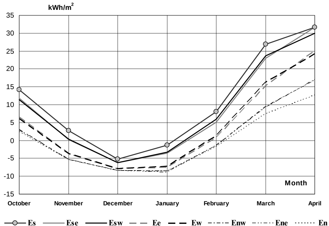
Fig. 4. Solar energy penetrating the building through its glazing of different orientations (sum of solar energy gains and heat losses). Es, Ese, Esw, Ee, Ew, Enw, Ene, En – energy balance of south, south east, south west, east, west, north west, north east and north glazing
