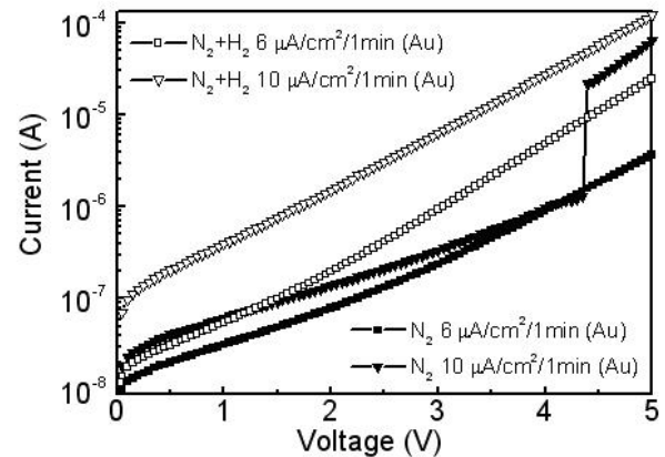
Fig. 3. Effects of \text{N}_2 + \text{H}_2 and \text{N}_2 ion beam nitridation on reverse I-V characteristics of Au-GaAs Schottky contacts (ion beam energy 65 eV, treatment time 1 min)
