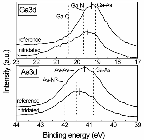
Fig. 5. Effects of GaAs surface nitridation on Ga3d and As3d XPS spectra (nitrogen ion beam energy 65 eV, ion beam current density 10 \mu\text{A}/\text{cm}^2 , irradiation time 1 min)
