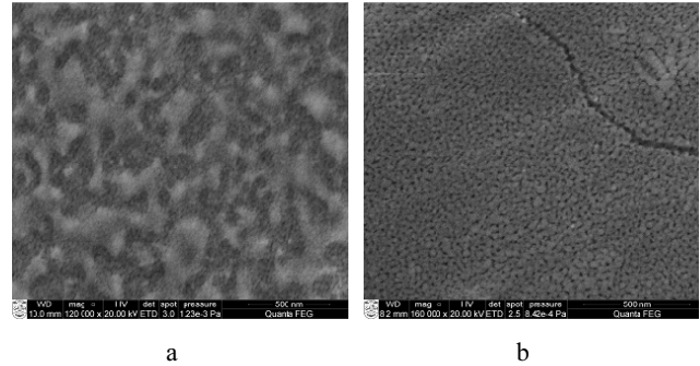
Fig. 4. SEM micrographs of YSZ thin films after different dipping counts and annealing procedures and prepared by the different synthesis route: (a) 7 dipping by the synthesis route (I), (b) 7 dipping by the synthesis route (II)
