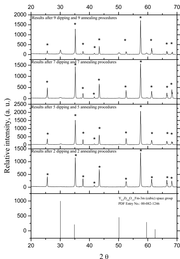
Fig. 2. XRD patterns of the YSZ samples annealed at 800 °C after each dipping procedure for 1 h in air (synthesis route (II)). * – characteristic peaks of the substrate ( \text{Al}_2\text{O}_3 ), (the last inset shows intensity distribution for \text{Y}_{0.2}\text{Zr}_{0.8}\text{O}_{1.9} for Fm-3m space group)
