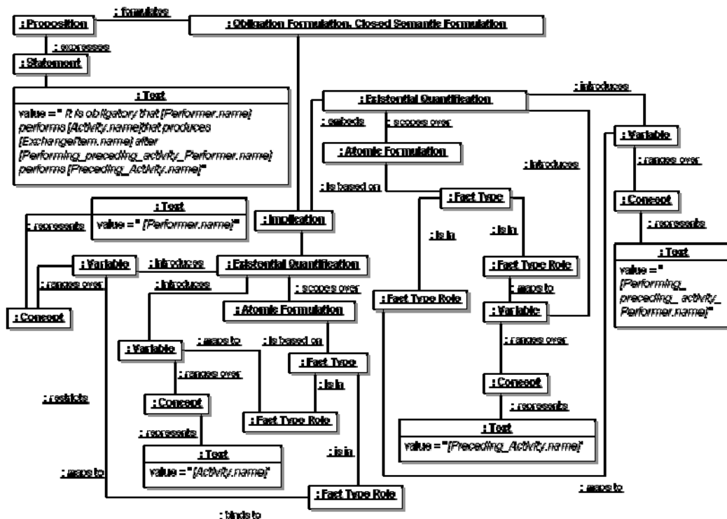
Figure 3. The example of the transformation pattern as the instance of SBVR MOF metamodel
