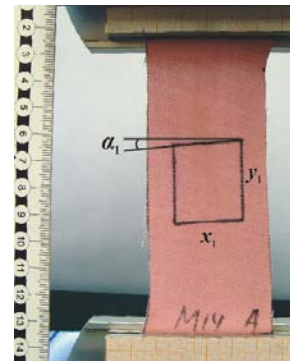
Fig 3. The specimen of fabric M14 cut in weft direction after ultimate extension \varepsilon = 4 %
