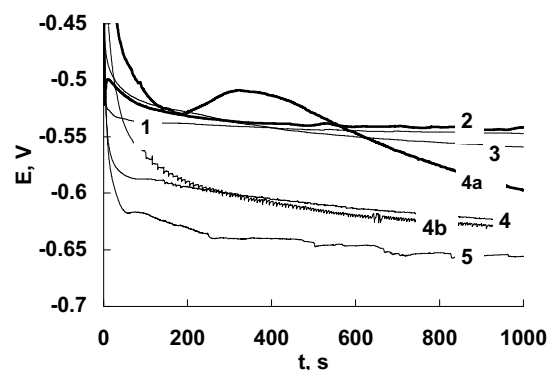
Fig. 2. OCP of Fe-electrode in 0.5\text{ M Na}_2\text{SO}_4 (pH 3.0) with various additions of \text{LiBH}_4 or \text{FeSO}_4 , (in \text{mol L}^{-1} ): 1 – 0; 2 – 0.018\text{ M FeSO}_4 ; 3 – 0.0072\text{ M LiBH}_4 ; 4 – 0.036\text{ M LiBH}_4 (IV); 4a – IV + 0.5\text{ wt\% OS-20} ; 4b – IV + 0.5\text{ wt\% Tetronic 90R4} ; 5 – 0.09\text{ M LiBH}_4
