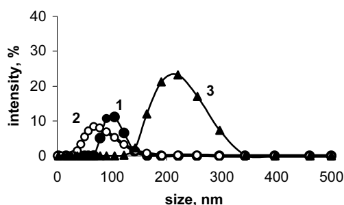
Fig. 8. The size distribution of Fe particles obtained in water with adding surfactants: OS-20 (1), Tetronic 90R4 (2) and without surfactant (3) in the presence of \text{NaBH}_4 . Resulting concentration of Fe particles is 0.1 wt %
