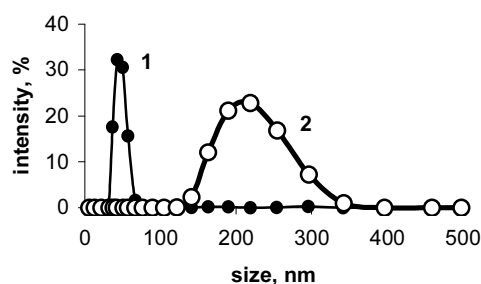
Fig. 4. The size distribution of Fe-particles obtained in aqueous solution in the presence of \text{LiBEt}_3\text{H} (1) and \text{NaBH}_4 (2). Resulting concentration of Fe-particles is 0.1 wt %
