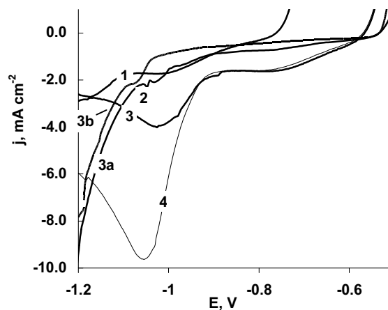
Fig. 3. Cathodic polarization curves of Fe-electrode in 0.5\text{ M Na}_2\text{SO}_4 solutions at pH 3 and containing various concentrations of \text{FeSO}_4 : 1 – 0; 2 – 0.0036\text{ M} ; 3 – 0.018\text{ M (III)} ; 3a – III + 0.5\text{ wt\% OS-20} ; 3b – III + 0.5\text{ wt\% Tetronic 90R4} ; 4 – 0.090\text{ M}
