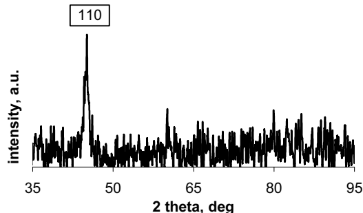
Fig. 6. XRD pattern of Fe powder followed synthesis by the reduction using \text{NaBH}_4 as reducing agent in water phase and dried at room temperature
