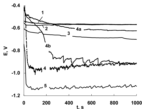
Fig. 1. OCP vs. immersion time of Fe-electrode in 0.5\text{ M Na}_2\text{SO}_4 (pH 3.0) with various additions of \text{NaBH}_4 or \text{FeSO}_4 , (in \text{mol L}^{-1} ): 1 – 0; 2 – 0.018\text{ M FeSO}_4 ; 3 – 0.0072\text{ M NaBH}_4 ; 4 – 0.036\text{ M NaBH}_4 (IV); 4a – IV + 0.5\text{ wt\% Tetronic 90R4} ; 4b – IV + 0.5\text{ wt\% OS-20} ; 5 – 0.18\text{ M NaBH}_4
