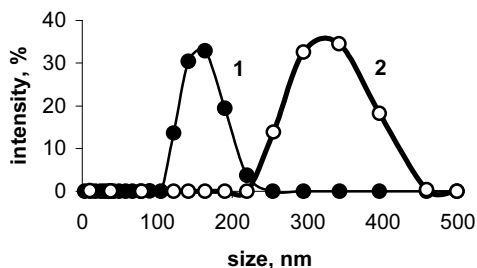
Fig. 5. The size distribution of Fe-particles obtained in the reverse micelles formed in the mineral SAE-10 oil in the presence of \text{LiBEt}_3\text{H} (1) and \text{NaBH}_4 (2). Resulting concentration of Fe-particles is 0.1 wt %
