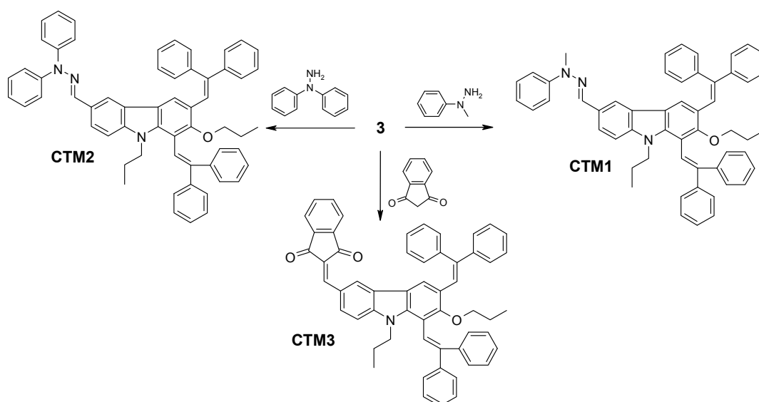
Scheme 2. Synthesis routes to charge-transporting materials CTM1–3 .
