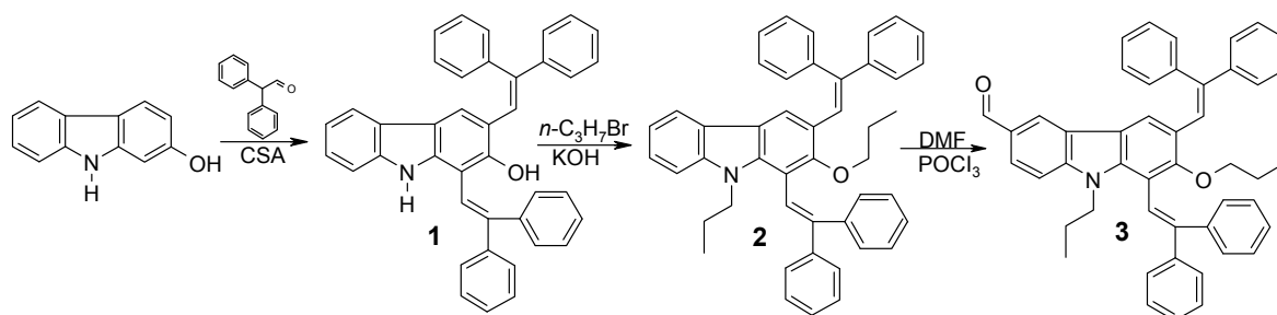
Scheme 1. Synthesis route to the aldehyde 3 .
