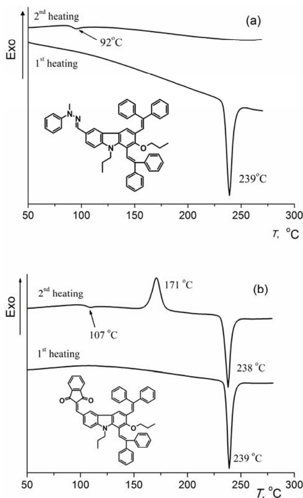
Figure 1. (a) DSC curves of CTM1 ; (b) DSC curves of CTM3 (heating rate 10 K/min).
