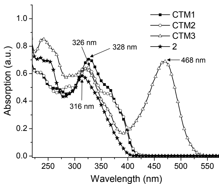
Figure 2. UV/Vis absorption spectra of 10^{-4} M THF solutions of CTM1–3 and 2 .
