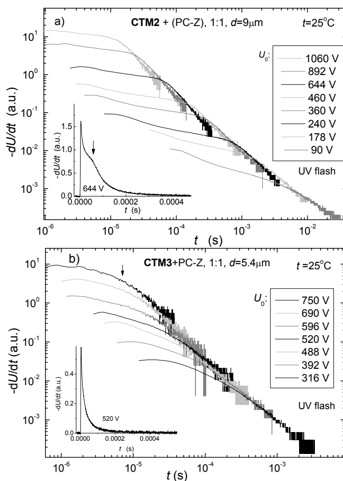
Figure 5. (a) XTOF transients for CTM2 (1:1 composition with PC-Z); (b) XTOF transients for CTM3 (1:1 composition with PC-Z).
