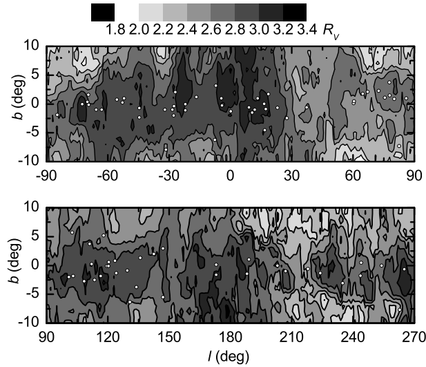
Fig. 1. 2D map of the distribution of the parameter R_V . Empty circles mark the location of OB associations (Ruprecht 1966).
