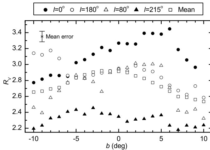
Fig. 2. The dependence of the parameter R_V on Galactic latitude for selected Galactic longitudes.
