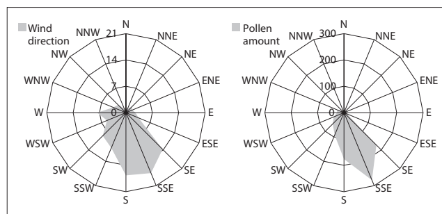
Figure 7. Wind rose during the pollen recording period (on the left) and the ratio (on the right) of pollen count in the air to wind direction
