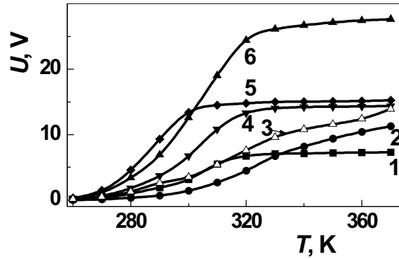
Fig. 1. Dependences of electret potential of Zn_{0.7}Cd_{0.3}S layers on the poling temperature at different poling electrical field: E = 17 (1), E = 68 (6) and E = 34 \text{ V}/\mu\text{m} (2–5); poling duration: t_p = 15 (1, 4, 6), t_p = 2 (2) and t_p = 60 \text{ min} (5). Layer thickness L = 3.0 \mu\text{m} .
