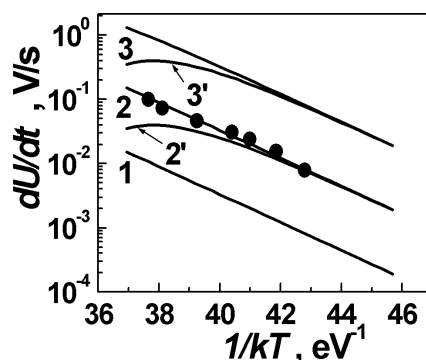
Fig. 2. Dependencies of the rates of thermodepolarisation on the temperature in the \text{Zn}_{0.7}\text{Cd}_{0.3}\text{S} layers ( \bullet ) as well as the results of computer simulation. It has been supposed in the model, that the effective density of states in the conductivity zone N_c is equal to: 2 \cdot 10^{23} (1), 2 \cdot 10^{24} (2), 2 \cdot 10^{25} \text{ m}^{-3} (3); recombination times: t_r = 10^{-3} (1–3), 10^{-4} (3') and 10^{-6} \text{ s} (2'); poling electrical field E = 5 \text{ V}/\mu\text{m} ; activation energy W_t = 0.5 \text{ eV} .
