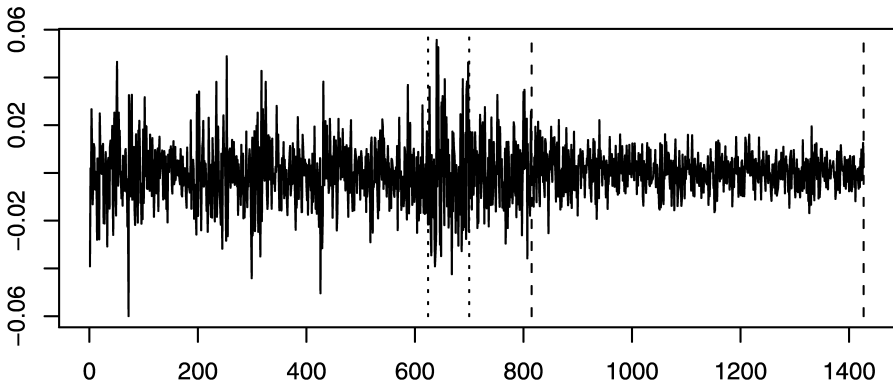
Fig. 1. Log-returns of S&P.
