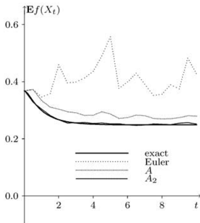
Fig. 2. Approximation of the CIR equation dX_t = (a - bX_t) dt + \sigma \sqrt{X_t} dB_t , a = b = 1 , \sigma = 1 , f(x) = \exp(-2x) , x_0 = 0.5 .
