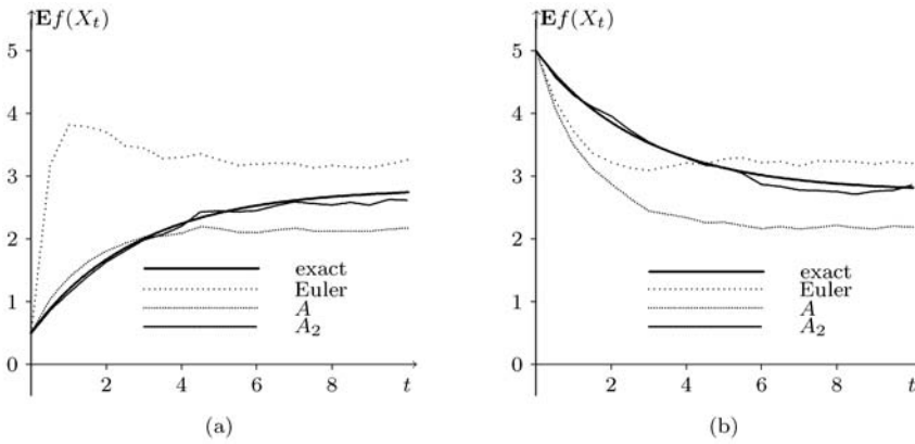
Fig. 1. Approximation of the stochastic Verhulst equation dX_t = \lambda X_t(1 - X_t) dt + \sigma X_t dB_t , \lambda = 1 , \sigma = 0.8 , f(x) = \frac{1}{x} ; (a) x_0 = 2 , (b) x_0 = 0.2 .
