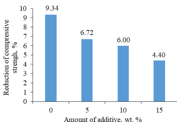
Figure 1. CMC additive effect on the compressive strength decrease level of the samples treated from 6 till 9 month in the 5 % Na 2 SO 4 solution.
