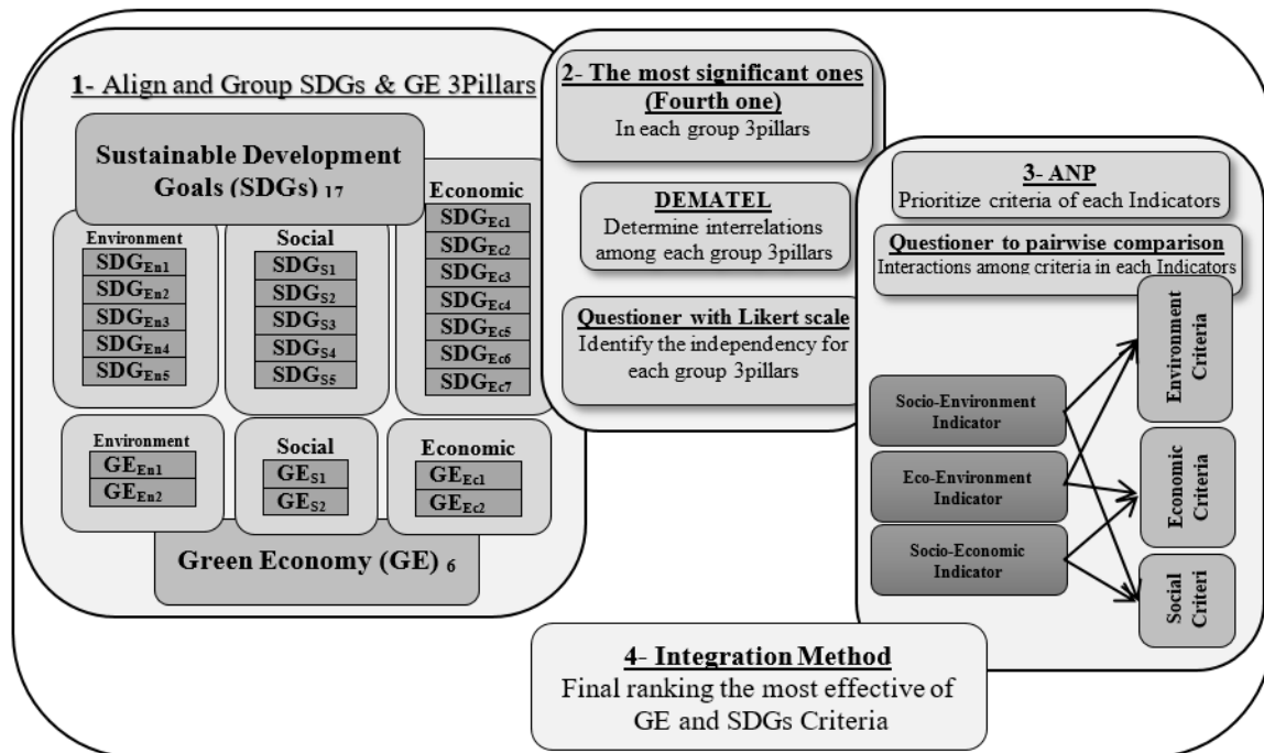
Figure 4. Research Framework.
