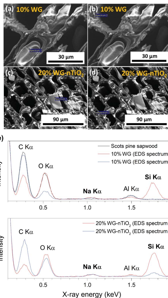
Fig. 8 (a-d) Cross-section FE-SEM images depicting EDS-analysed regions, and (e) EDS spectra of 10% Na-O-Si and 20% Na-O-Si- n\text{TiO}_2 treated Scots pine sapwood.
