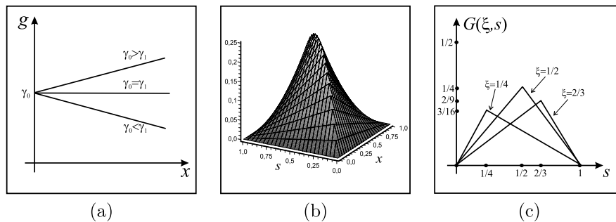
Fig. 1. (a) Function g = \gamma_0 + x(\gamma_1 - \gamma_0) ; (b) classical Green's function; (c) function G^{cl}(\xi, s) .
