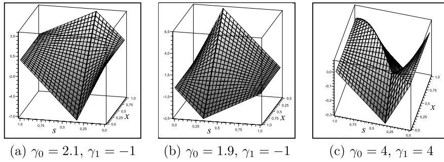
Fig. 3. Graphs of Green's function with \xi_0 = \xi_1 = 1/3 .
