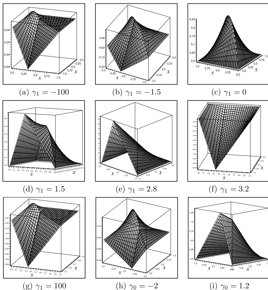
Fig. 2. Graphs of Green's function with \xi_0 = \xi_1 = 1/3 and (a)–(g) \gamma_0 = 0 and various \gamma_1 = -100, -1.5, 0, 1.5, 2.8, 3.2, 100 ; (h)–(i) \gamma_1 = 0 and various \gamma_0 = -2, 1.2 .
