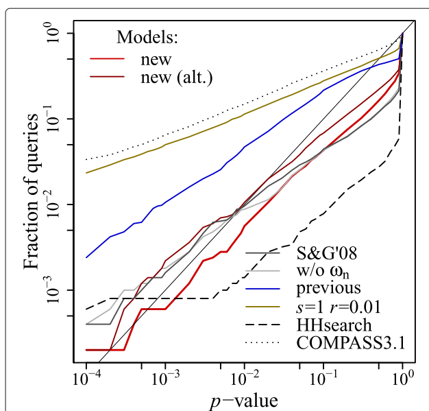
Fig. 4 Statistical accuracy of the COMER method using different models for statistical significance estimation. Shown are the results of comparing the profiles constructed for 5000 randomized Pfam families to the profiles constructed for 4931 randomized SCOPe domains. The figure plots the fraction of queries with a p -value reported for their best match less than the p -value indicated on the x -axis. The solid straight line indicates the highest accuracy. These models are represented in the figure: the new model (new) proposed, the alternative model with E -value correction (new (alt.)), a statistical model based on previous research (S&G'08), the statistical model used in the previous COMER version (previous), a model based on the statistics obtained for profiles generated with s = 1 and r = 0.01 , and the model excluding the number of positive substitution scores (w/o \omega_n ). The statistical accuracy of HHsearch and COMPASS (v3.1) is also shown
