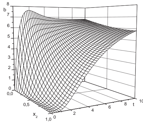
Fig. 3. Graph of function b(t, 0, x_2) from system (1)–(3) for k_f = 1, k_r = 0.1, k = 1 .
