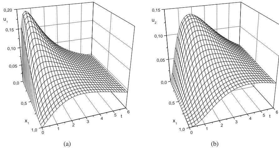
Fig. 6. Graph of functions (a) u_1(t, x_1) , (b) u_2(t, x_1) from system (4)–(6) for k_f = 0.2 , k_r = 1 , k_{r1} = 1 , k = 1 .
