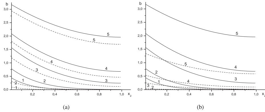
Fig. 2. Graphs of function b(t, 0, x_2) from systems (1)–(3) (solid line) and (4)–(6) (dash) for k_f = 0.2, k_r = 1, k = 0.1 , (a) k_{r1} = 1 , (b) k_{r1} = 0.1 : 0.5 – curves 1, 1 – curves 2, 3 – curves 3, 5 – curves 4, 10 – curves 5.
