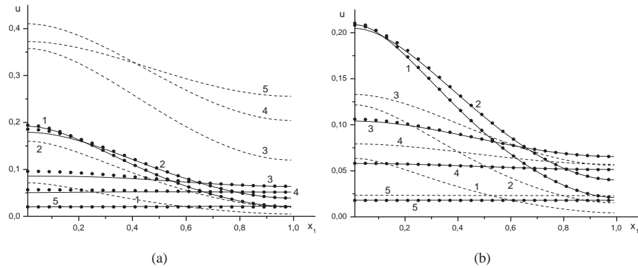
Fig. 5. Graphs of functions u(t, 0, x_1) (bullets) from system (1)–(3) and u_1(t, 0, x_1) (solid line), u_2(t, 0, x_1) (dash) from system (4)–(6) for k_f = 0.2 , k_{r1} = 0.1 , k = 1 , (a) k_r = 1 , (b) k_r = 0.01 , and t : 0.5 – 1, 1 – 2, 3 – 3, 5 – 4, 10 – 5.
