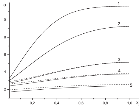
Fig. 1. Graphs of function a(t, 0, x_2) from systems (1)–(3) (solid line) and (4)–(6) (dash) for k_f = 0.2, k_r = 1, k_{r1} = 0.1, k = 0.1: 0.5 – curves 1, 1 – curves 2, 3 – curves 3, 5 – curves 4, 10 – curves 5.
