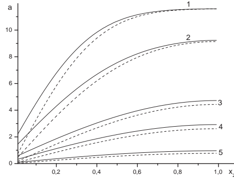
Fig. 4. Graphs of function a(t, 0, x_2) from system (4)–(6) for k_r = 0.1 , k_{r1} = 1 , k = 1 , k_f = 0.2 (solid line) and k_f = 1 (dash), and t : 0.5 – curves 1, 1 – curves 2, 3 – curves 3, 5 – curves 4, 10 – curves 5.
