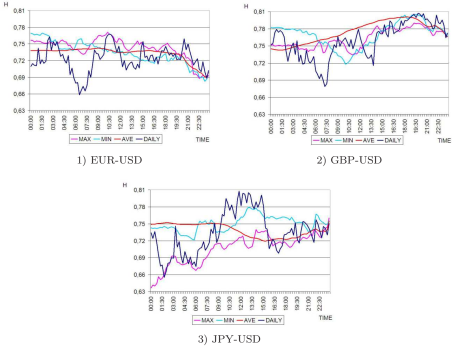
Fig. 1. Hurst exponents dependence on data aggregation.
