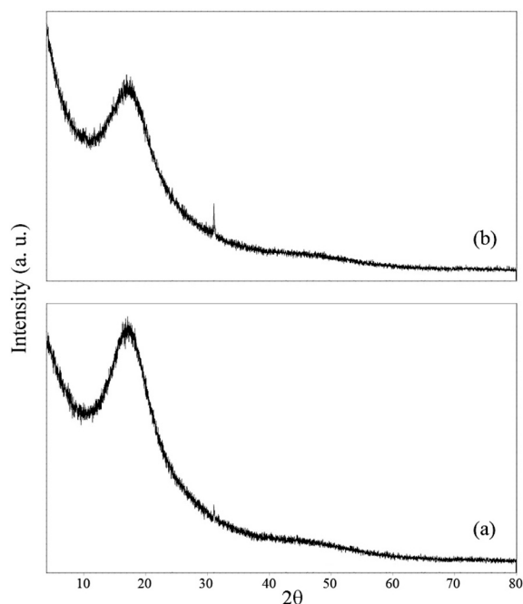
Fig. 5. XRD patterns of archaeological amber samples from villages Benaičiai (a) and Turlojiškės (b).
