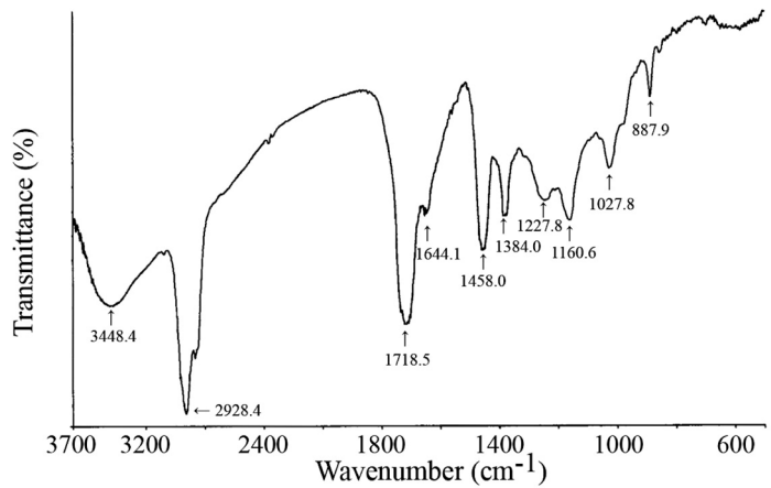
Fig. 3. FTIR spectrum of amber sample found in old town of Vilnius.
