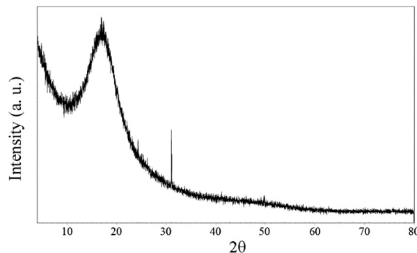
Fig. 6. XRD pattern of amber sample found in old town of Vilnius.
