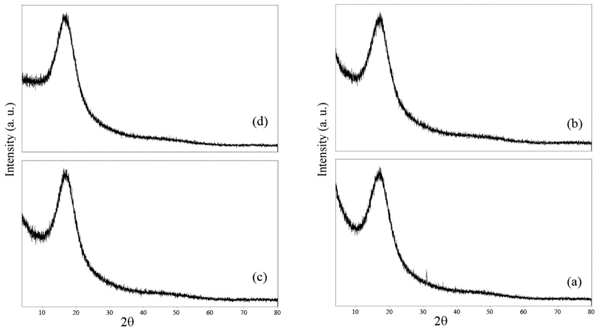
Fig. 4. XRD patterns of milky (a), dark (b), opaque (c) and transparent (d) amber samples from Baltic Coast in Nida.
