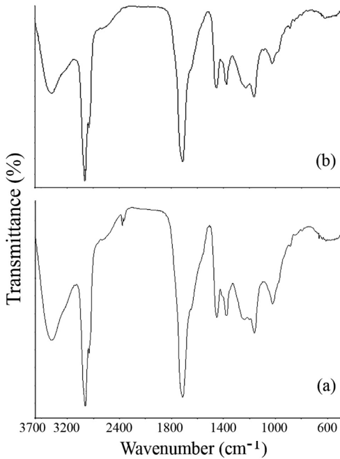
Fig. 2. FTIR spectra of archaeological amber samples from villages Benaičiai (a) and Turlojiškės (b).
