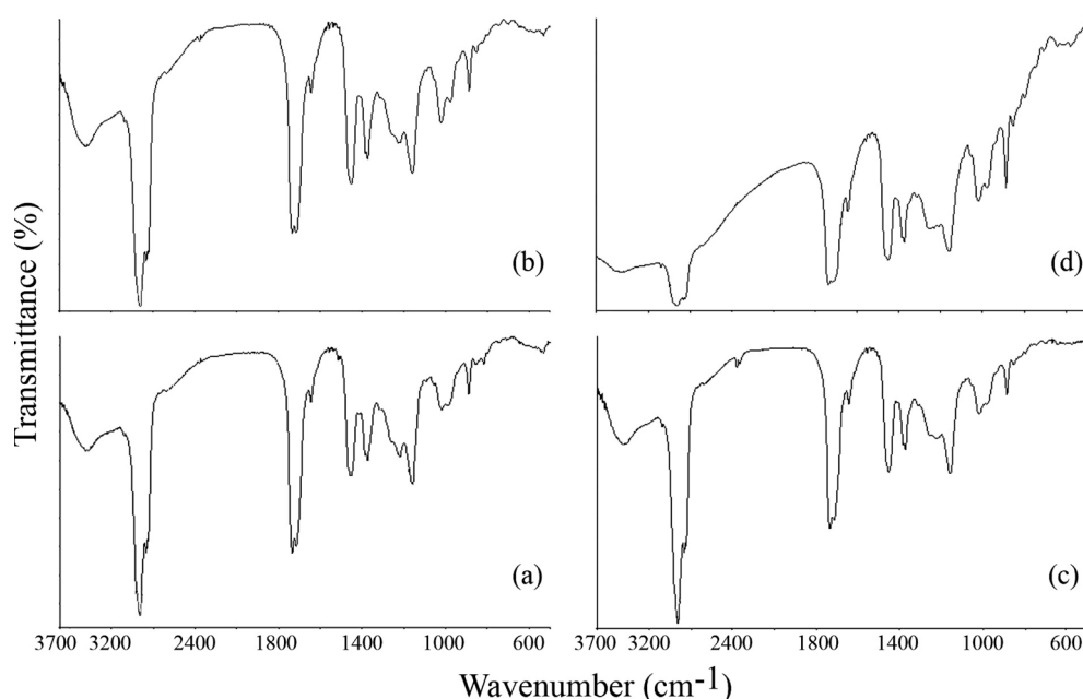
Fig. 1. FTIR spectra of milky (a), dark (b), opaque (c) and transparent (d) amber samples from Baltic Coast in Nida.
