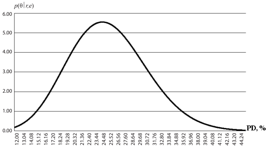
FIG. 6. Posterior distribution of PD for rating 7 in 2007
