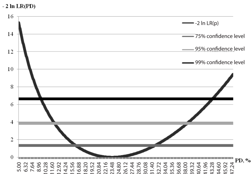
FIG. 4. Estimation of PD_{2007} for rating 7
