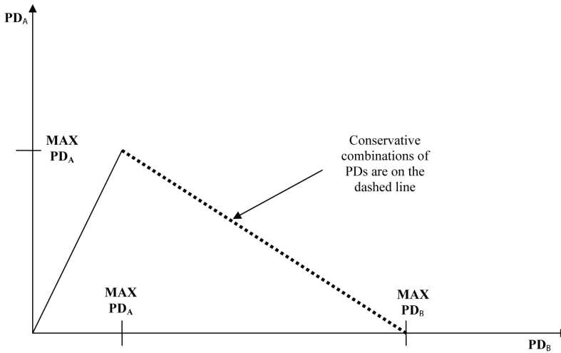
FIG. 2. Estimation of PDs for several LDP ratings with no actual defaults
