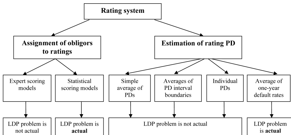
FIG. 1. LDP problem
