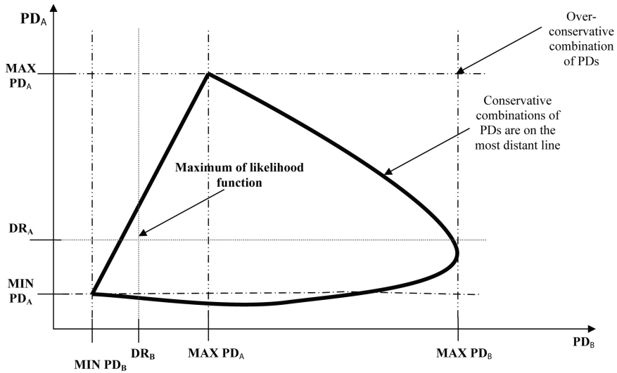
FIG. 3. Estimation of PDs for several LDP ratings with several actual defaults
