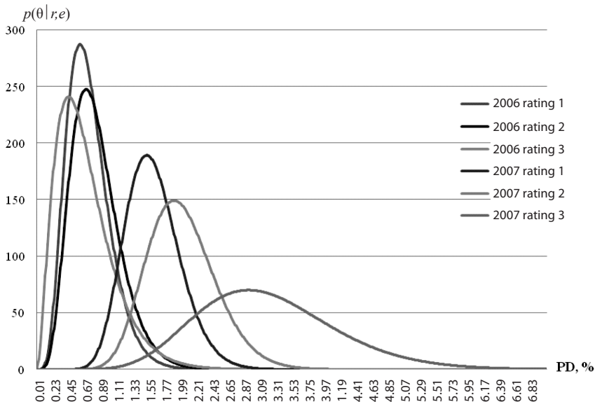
FIG. 5. Posterior distributions of PDs for ratings 1, 2 and 3 in 2006 and 2007
