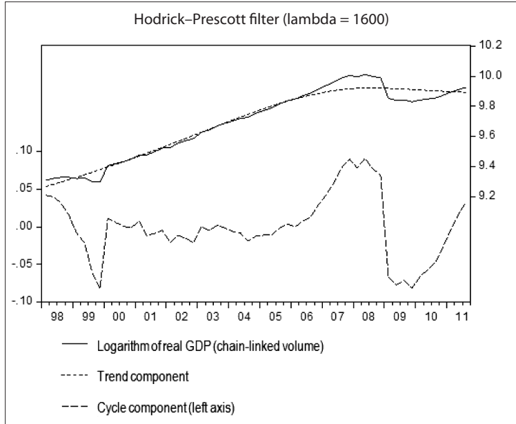
FIG. 1. Decomposition of chained-volume GDP of Lithuania into trend and cyclical components using HP filter, 1998 Q1 – 2011 Q3
