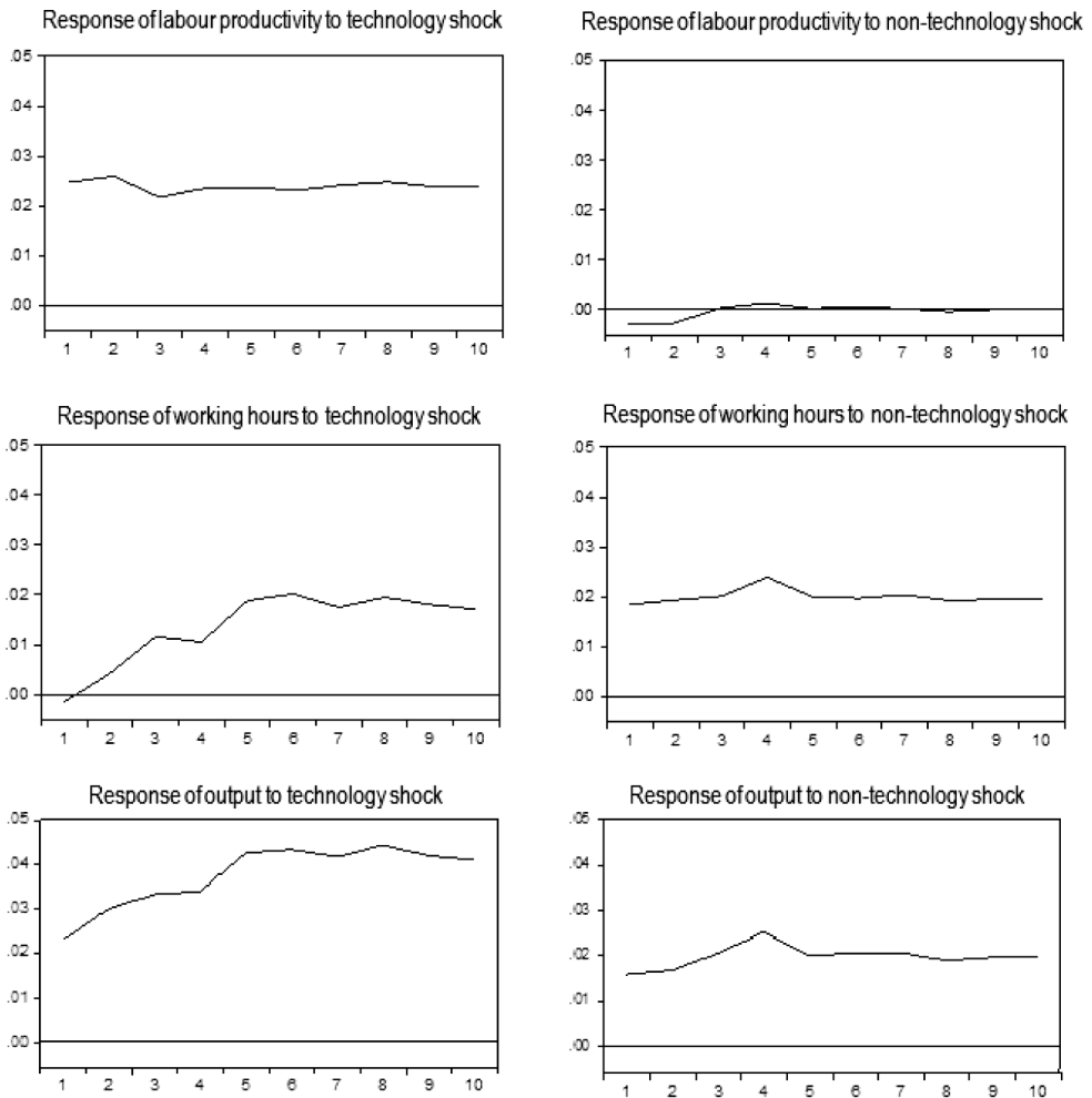
FIG. 4. Impulse-responses of labour productivity, working hours and output to technology and non-technology shocks of 1-standard deviation
