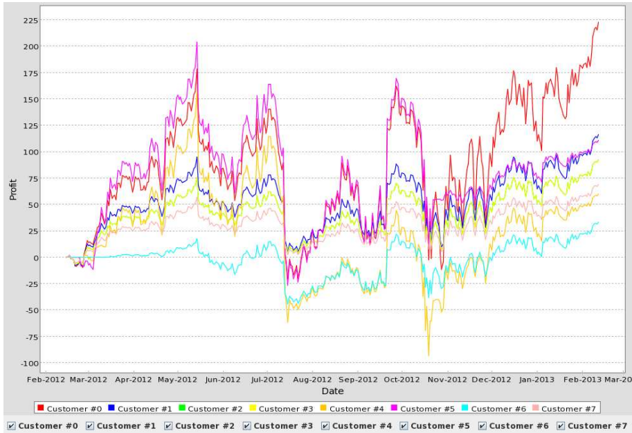
Fig. 1. Daily profits of eight customers buying-selling Nike stocks.
