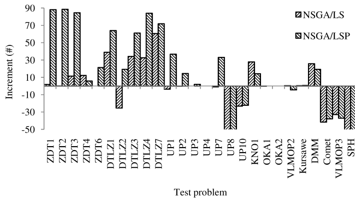
Fig. 9. Improvement in units of performance metric C .
