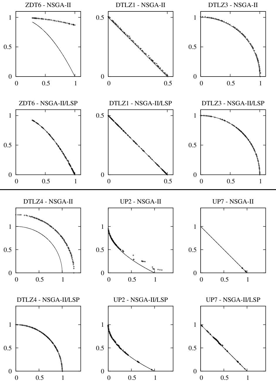
Fig. 10. Illustration of approximations of Pareto fronts of several test functions, obtained by NSGA-II and NSGA/LSP.
