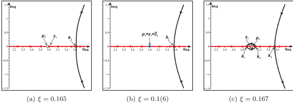
Fig. 6. The domain \mathcal{N} of CFs in the neighborhood of the second type constant eigenvalue point.
