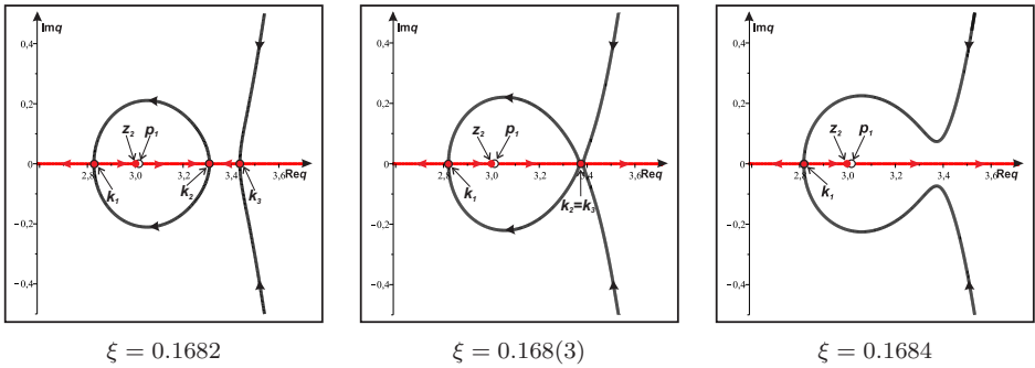
Fig. 7. The domain \mathcal{N} of CFs in the neighborhood of the critical point of the second order.
