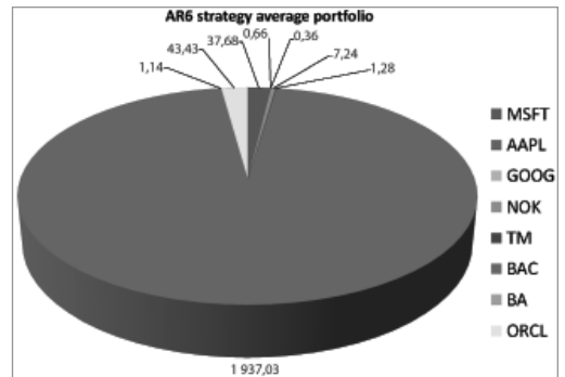
Fig. 4. The most profitable portfolio defined using the first strategy and AR(6) prediction model
