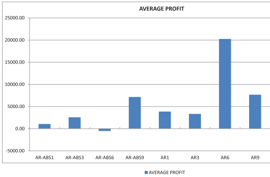
Fig. 2. Average profits of eight prediction models by the first strategy using historical data
