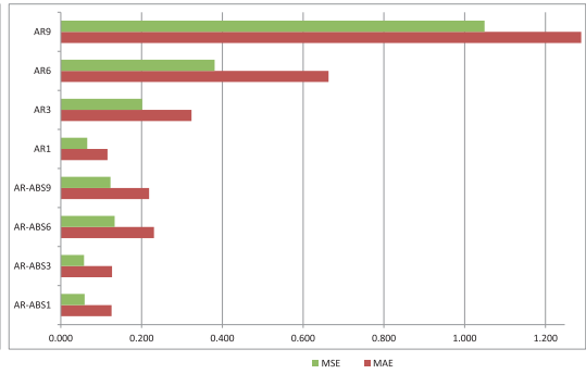
Fig. 3. Average prediction errors using different prediction models
