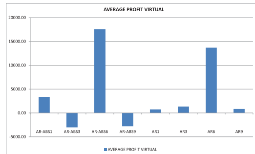
Fig. 1. Average profits of eight prediction models by the first strategy using virtual data
