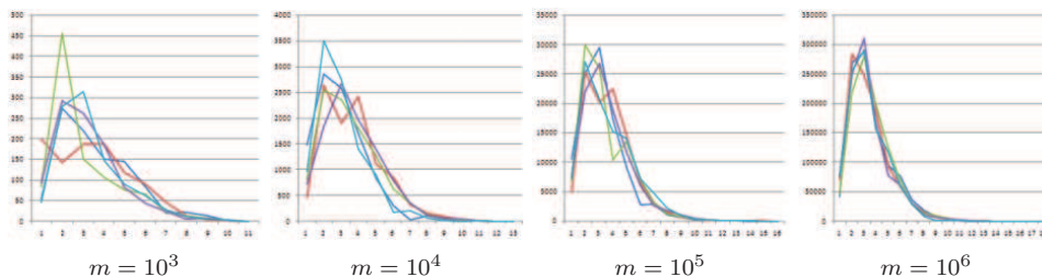
Fig. 1. Convergence to Nash equilibrium.
