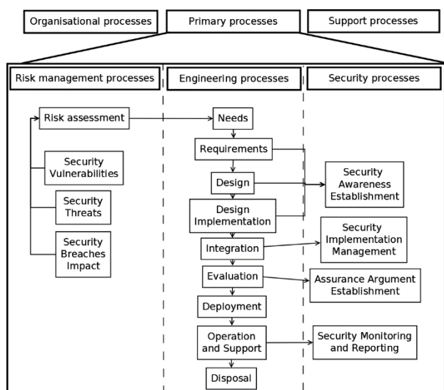
Fig. 1. Information Security Process Capability Model: relationship of the Primary Process category processes.
