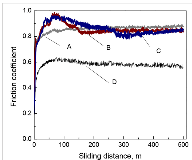
FIGURE 7 | Evolution of the coefficient of friction of Fe-W (A) and Fe-W/Al 2 O 3 composite coatings obtained with different concentration of alumina in electrolyte: 25 g L -1 (B), 50 g L -1 (C), and 100 g L -1 (D) tested under dry friction conditions at 2 N load, 4 cm s -1 , 500 m.
