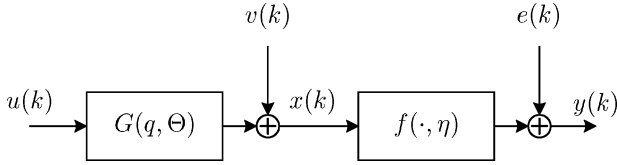
Fig. 1. The PWA system with the process noise v(k) and that of the measurement e(k) . The linear dynamic part G(q, \Theta) of the PWA system is parameterised by \Theta , while a static nonlinear part f(\cdot, \eta) – by \eta . Signals: u(k) is input, y(k) is output, x(k) is an unmeasurable intermediate signal.
