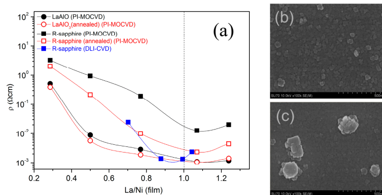
Figure 7. (a) Composition dependence of resistivity of as-deposited and annealed (at 750 °C) \text{LaNiO}_3 films on \text{LaAlO}_3 and R-sapphire substrates grown by PI-MOCVD at 600 °C and by DLI-CVD at 750 °C. The resistivity SEM image of \text{LaNiO}_3 film morphology with (b) \text{La}_2\text{O}_3 -poor ( \text{La}/\text{Ni} = 0.9 ) and (c) \text{La}_2\text{O}_3 -rich ( \text{La}/\text{Ni} = 1.02 ) compositions.
