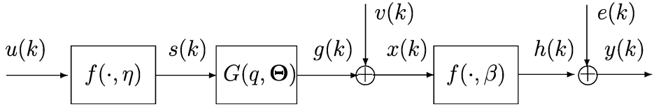
Fig. 1. The block-oriented H-W system with the process noise v(k) and that of the measurement e(k) . The linear dynamic part G(q, \Theta) of the H-W system is parameterised by \Theta , while the static nonlinear parts f(\cdot, \eta) – by \eta and f(\cdot, \beta) – by \beta . Signals: u(k) is input, y(k) is output, s(k) , g(k) , x(k) , h(k) are unmeasurable intermediate signals.
