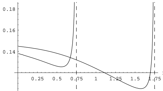
Fig. 2. The graphs of \tilde{\sigma}_p^2(H) , p = 1, 2 .
