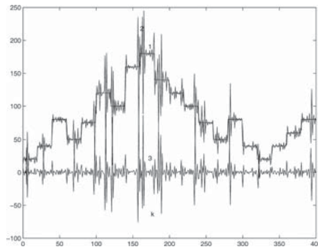
Fig. 2. Signals of a noisy closed-loop system in the presence of outliers in v(k) ( \epsilon = 0.1 ): 1) the reference signal r(k) , 2) the output y(k) corrupted by an additive noise with outliers in it, 3) the input u(k) .
