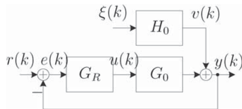
Fig. 1. A closed-loop system to be observed. Here G_R \equiv G_R(q^{-1}; \alpha) G_0 \equiv G_0(q^{-1}; \theta) , and H_0 \equiv H_0(q^{-1}; \varphi) .
