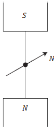
Figure 2.3: Detection of the direction of the electron
