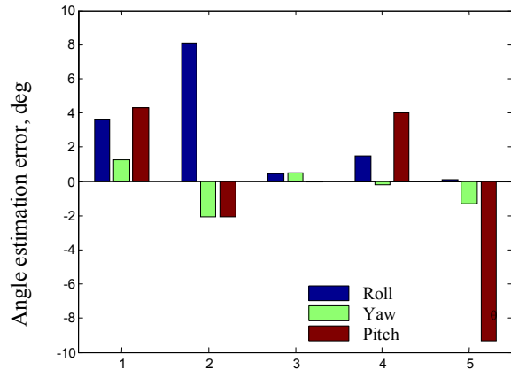
Fig. 3. Mean angle estimation error without expression compensation after head rotation about three axis by 10 degrees
