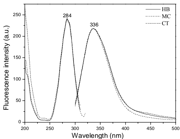
Fig. 2. Fluorescence excitation spectra ( \lambda_{\text{d}} = 335 ) nm and fluorescence spectra ( \lambda_{\text{ex}} = 280 ) nm of HB, MC and CT homogenates (first soluble fraction) normalized at 284 nm and 336 nm, respectively
