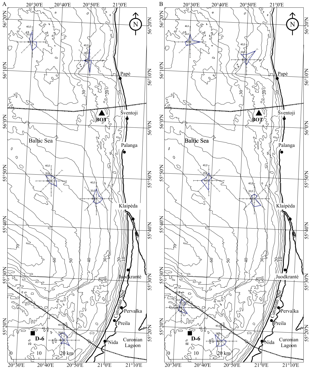
Figure 7. 5 m-layer current direction frequency (%) for the Baltic Sea: A) warm season, B) cold season.
