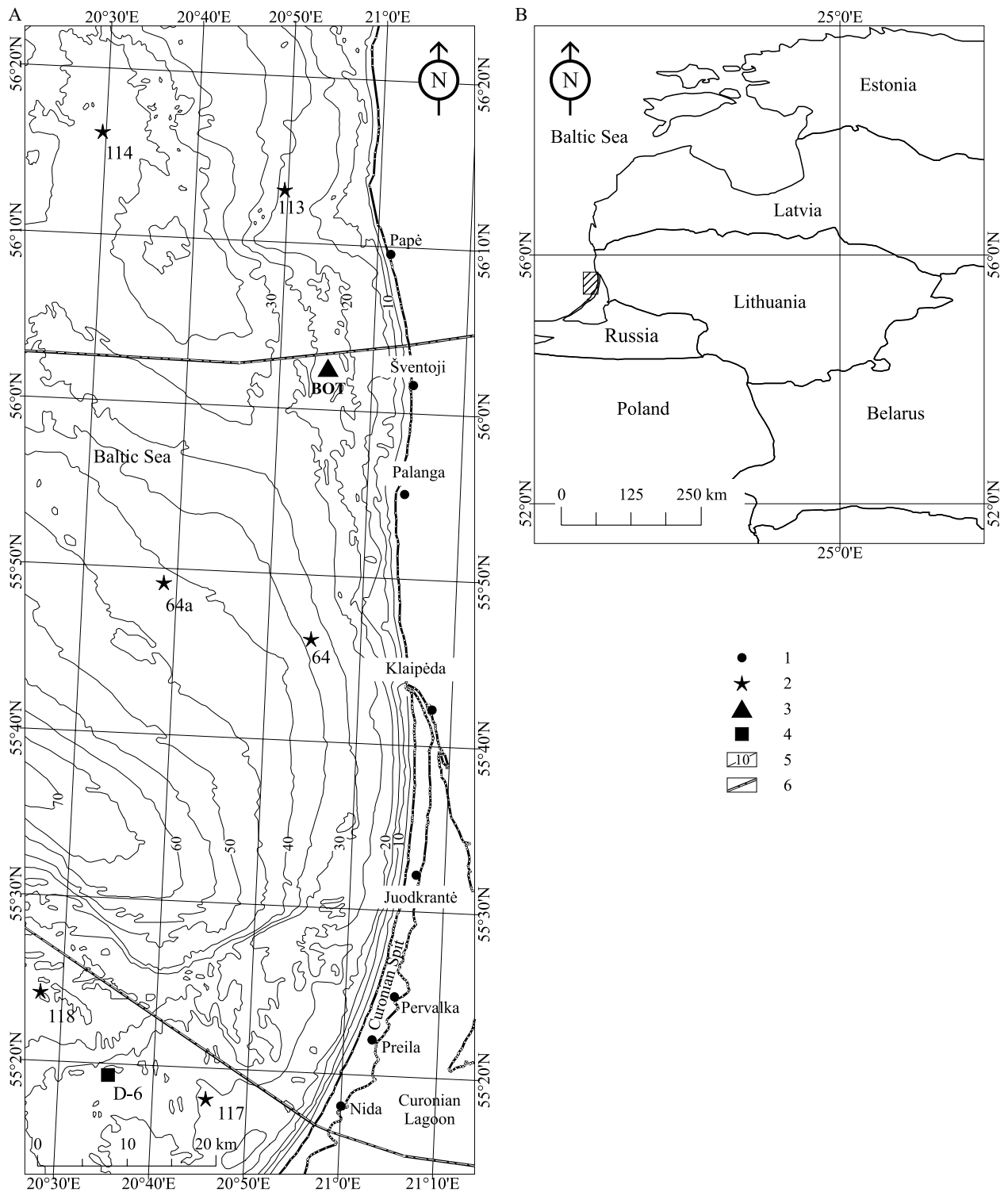
Figure 1. The map of the study area: 1 – settlement, 2 – oceanographic station, 3 – Būtingė Oil Terminal (BOT), 4 – Kravtsovskoje oil platform (D-6), 5 – isobaths, 6 – national border.
