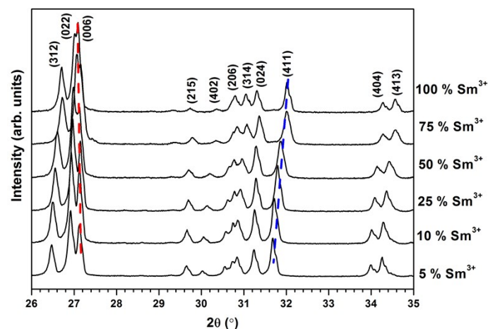
20 21 Figure S1. Fragment of XRD patterns of K_2Bi(PO_4)(MoO_4):Sm^{3+} as a function of Sm 3+ 22 concentration. 23
