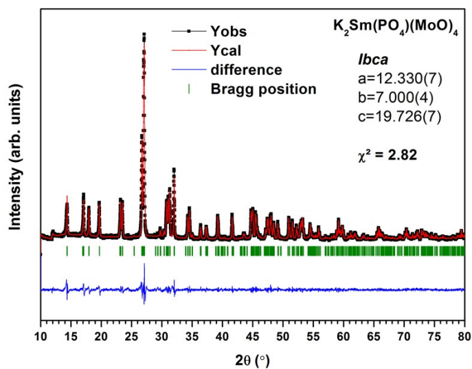
6 Figure S3. Rietveld refinement of K_2Sm(PO_4)(MoO_4) powder XRD pattern.
