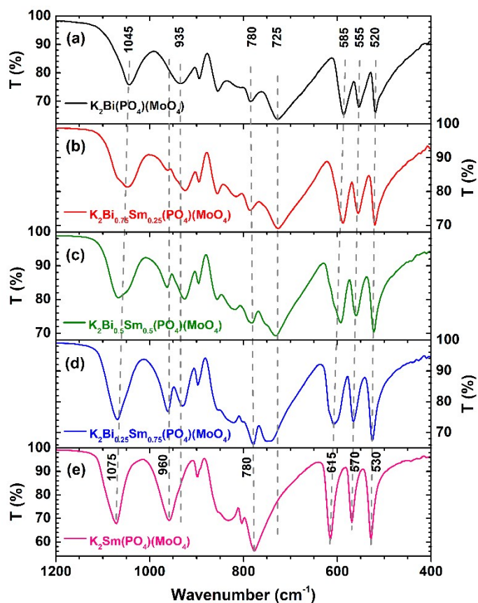
3 Figure S4. FTIR spectra of \text{K}_2\text{Bi}(\text{PO}_4)(\text{MoO}_4) doped with (a) 0%, (b) 25%, (c) 50%, (d) 75% and 4 (e) 100% \text{Sm}^{3+} .
