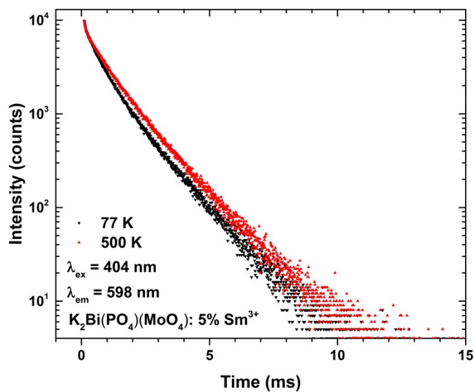
7 Figure S5. PL decay curves of \text{K}_2\text{Bi}(\text{PO}_4)(\text{MoO}_4):5\%\text{Sm}^{3+} as a function of temperature.
