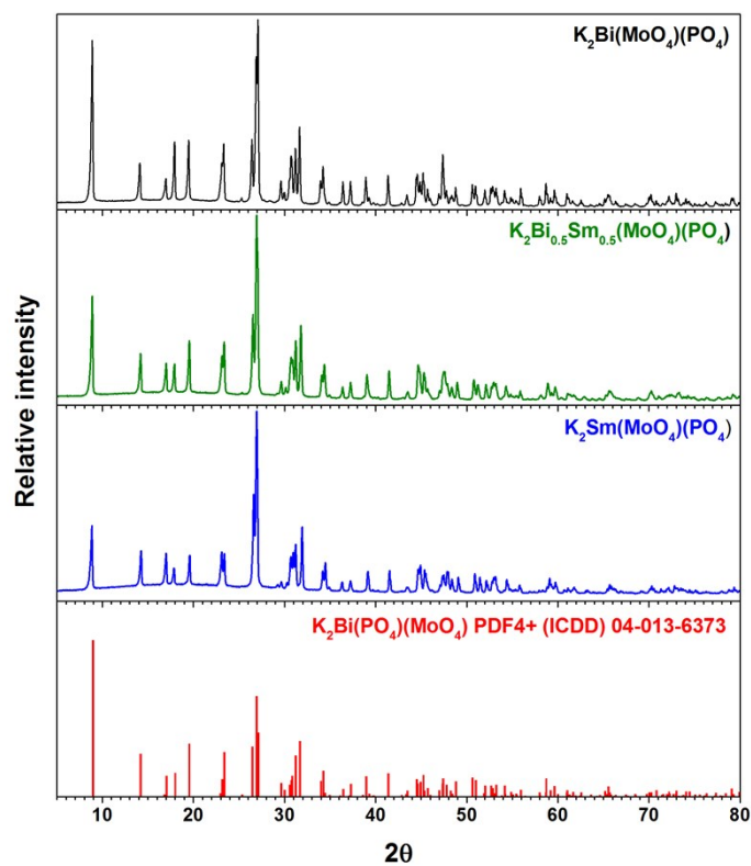
3 Figure S2. XRD patterns of K_2Bi(PO_4)(MoO_4):Sm^{3+} as a function of Sm^{3+} concentration.
