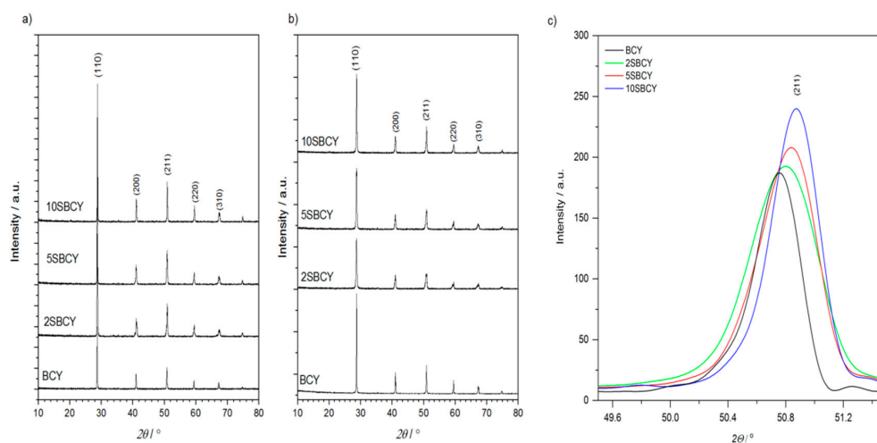
Figure 1. XRD patterns collected for Ba 1-x Sr x Ce 0.9 Y 0.1 O 3-δ (0 < x < 0.1) (SBCY) powders (a), sintered samples (b), and diffraction peak (211) shifts of SBCY samples toward greater diffraction angles (c) vs. chemical composition.
