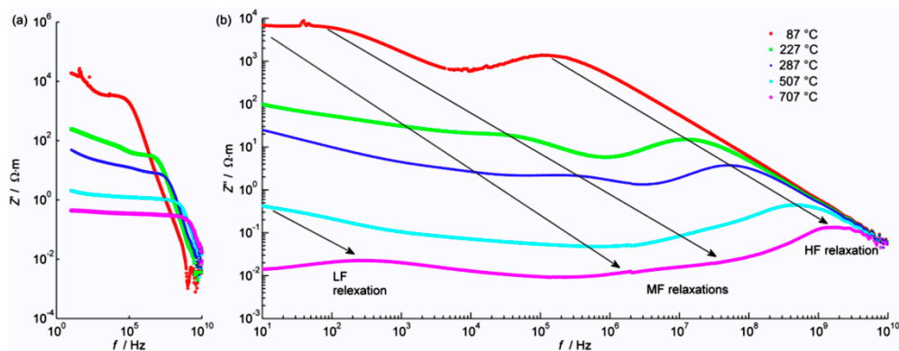
Figure 9. Spectra of (a) real Z' and (b) imaginary Z'' parts for a 2SBCY sintered pellet. Arrows indicate (approximately) the shift of the relaxation frequency of several processes with changes in temperature.
