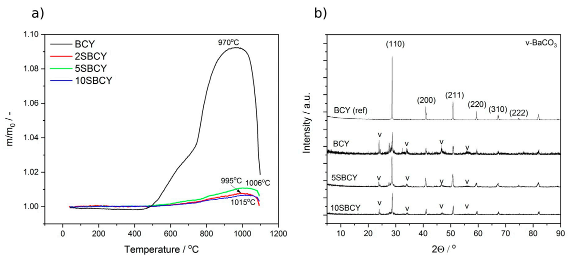
Figure 7. TG curves recorded for \text{Ba}_{1-x}\text{Sr}_x\text{Ce}_{0.9}\text{Y}_{0.1}\text{O}_{3-\delta} samples in a pure \text{CO}_2 gas atmosphere, at temperatures ranging from 25 to 1100^\circ\text{C} (a); XRD pattern recorded for SBCY samples after heating in 5 vol.% \text{CO}_2 in an Ar gas atmosphere at 550^\circ\text{C} for 100 h (b).
