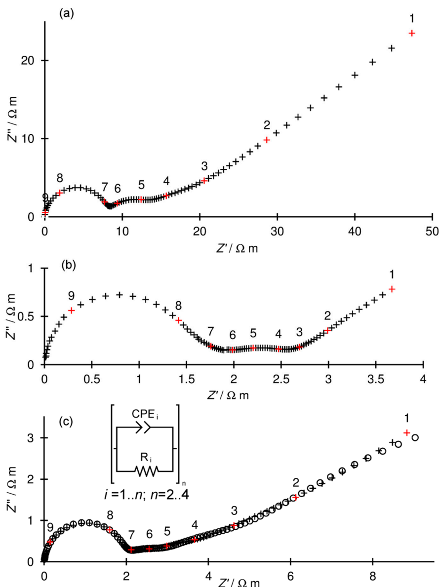
Figure 8. Complex impedance plane plots measured in air (a) at 287 °C for 2SBCY ceramics and (b) at 507 °C for 5SBCY ceramics; (c) an example of fit for 2SBCY ceramics measured at 407 °C; crosses indicate measured data, circles indicate the fitted model; numbers above red symbols denote logarithms of frequency.
