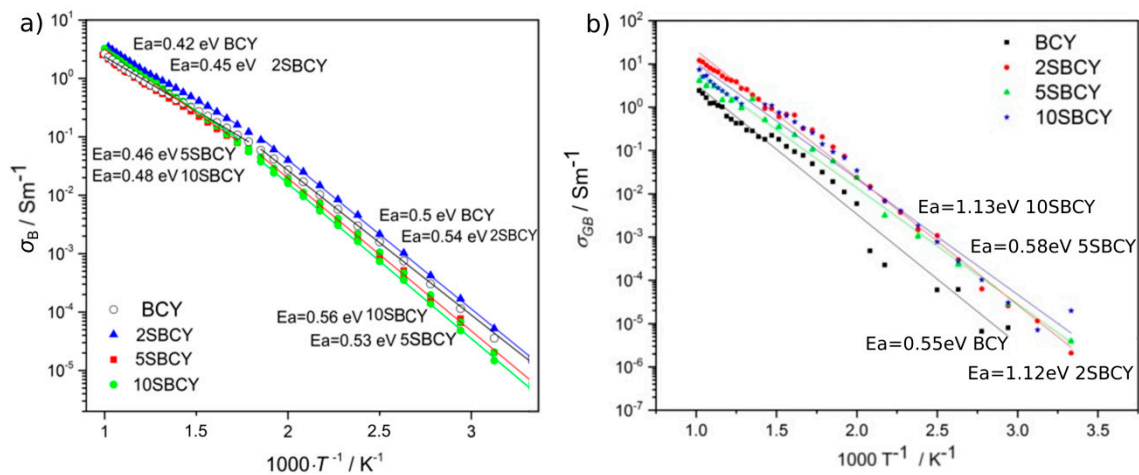
Figure 10. Variation in grain interior \sigma_B (a) and grain boundary \sigma_{GB} (b) conductivities of the SBCY sample series vs temperature.
