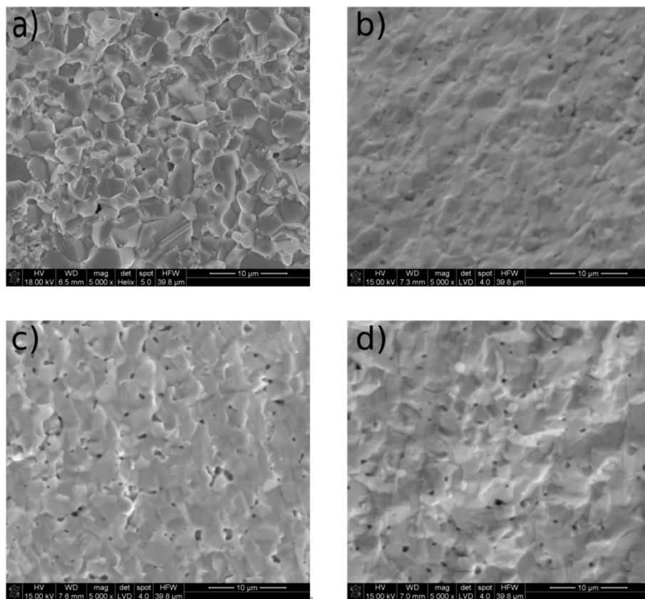
Figure 6. The microstructure of the representative surface of sintered (a) BCY, (b) 2SBCY, (c) 5SBCY, and (d) 10SBCY samples.
