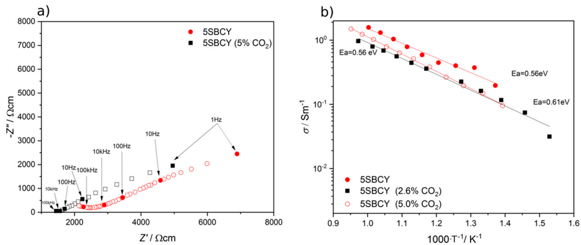
Figure 12. Impedance spectra ( Z'' – Z' ) recorded for the 5SBCY sample before and after additional heating in a 5 vol.% CO 2 gas atmosphere at 390 °C (a); variation in \sigma vs temperature recorded for 5SBCY before and after additional exposure in 5 or 2.6 vol.% CO 2 (b).
