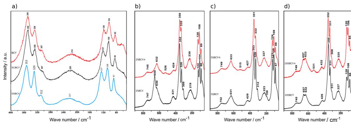
Figure 4. Raman spectra recorded for BCY (a), \text{Ba}_{0.98}\text{Sr}_{0.02}\text{Ce}_{0.9}\text{Y}_{0.1}\text{O}_{3-\delta} (2SBCY) (b), 5SBCY (c), and \text{Ba}_{0.9}\text{Sr}_{0.1}\text{Ce}_{0.9}\text{Y}_{0.1}\text{O}_{3-\delta} (10SBCY) (d) samples before and after additional heating (h) in 5 vol.% \text{H}_2\text{O-Ar} at 550\text{ }^\circ\text{C} for 100 h.
