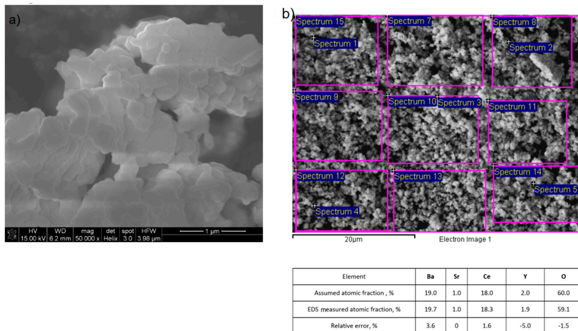
Figure 5. The representative SEM image recorded for 5SBCY powder (a) and SEM/EDS chemical analysis (b) performed for this sample.
