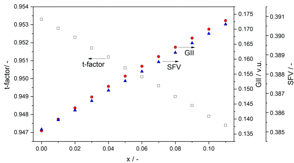
Figure 3. Dependence of the t tolerance factor, specific free volume SFV, and global instability index GII vs strontium content in \text{Ba}_{1-x}\text{Sr}_x\text{Ce}_{0.9}\text{Y}_{0.1}\text{O}_{3-\delta} samples.
