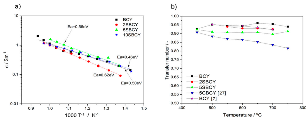
Figure 11. Independence of total electrical conductivity \sigma for SBCY sample series vs temperature recorded in \text{H}_2\text{O} -5 vol.% \text{H}_2 in Ar (a); variation in the t_{\text{ion}} transference number of BCY and 5SBCY ceramics determined by means of EMF measurements of a hydrogen concentration cell (b).
