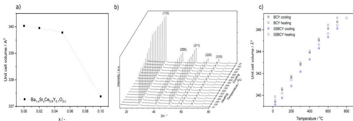
Figure 2. Variation in the cell volume of \text{Ba}_{1-x}\text{Sr}_x\text{Ce}_{0.9}\text{Y}_{0.1}\text{O}_{3-\delta} vs chemical composition at RT (a); XRD patterns collected for \text{Ba}_{0.95}\text{Sr}_{0.05}\text{Ce}_{0.9}\text{Y}_{0.1}\text{O}_{3-\delta} (5SBCY) during the heating-cooling cycle within the temperature range 25–800 °C (b) variation in \text{BaCe}_{0.9}\text{Y}_{0.1}\text{O}_{3-\delta} (BCY) and 5SBCY cell volume vs temperature (c).
