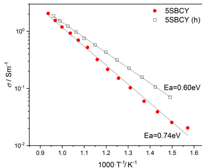
Figure 13. Variation \sigma vs 1000/T recorded for the 5SBCY sample before or after additional exposure in 5 vol.% H 2 O in Ar (h).
